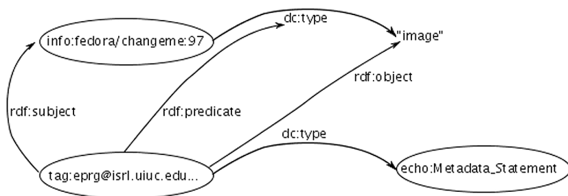
Figure 3. BECHAMEL has identified the fragment as a metadata statement
