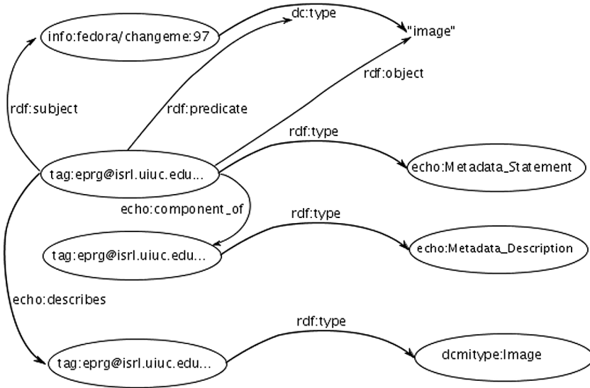
Figure 4. BECHAMEL has identified the metadata statement as a description of an image
