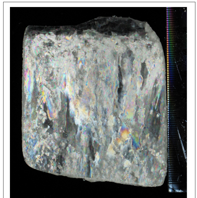
FIGURE 2 | An ice section (0.5 cm thick) of artificial sea ice from the low-Fe ice tank. An ice block (5 cm \times 10 cm \times 5.5 cm) was sectioned to 0.5 cm with a band saw at -20^{\circ}\text{C} . After planing with a microtome blade, the thick section was photographed between cross-polarized filters.
