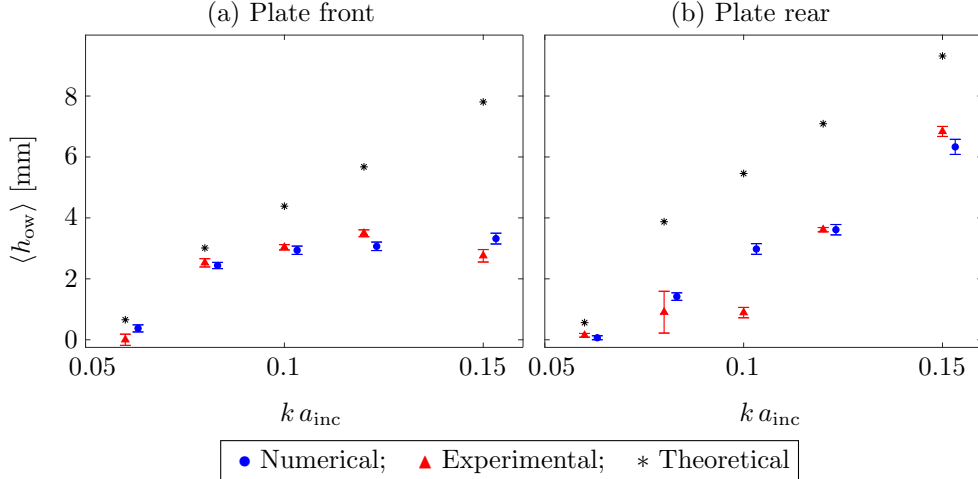
Figure 8: Overwash depth vs. incident steepness at (a) front end and (b) rear end of thin plate, with T_{\text{inc}} = 0.9 s, including predictions from theoretical model of Skene et al. (2015). Mean values (symbols) and two-times the standard deviations (error bars) are shown. Horizontal offsets \pm 0.002 are included for clarity.
