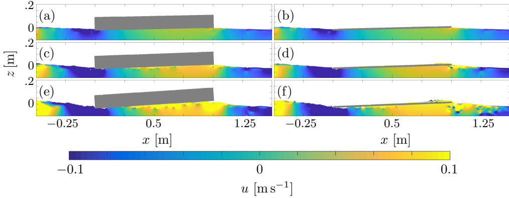
Figure 3: Horizontal velocity field u(x, z, t) around (a,c,e) thick plate and (b,d,f) thin plate, created by incident waves with period T_{\text{inc}} = 0.9 s and steepness (a,b) ka_{\text{inc}} = 0.06 , (c,d) 0.1, and (e,f) 0.15. Results produced by OpenFOAM post-processing tool ParaView. Movies S3–S4 show corresponding simulations.
