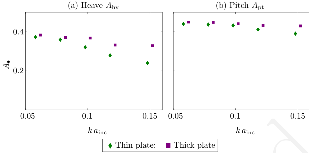
Figure 9: Response amplitude operators vs. incident steepness, where T_{inc} = 0.9 s, for (a) heave and (b) pitch, comparing thin plate (green diamonds) and thick plate (purple squares).
