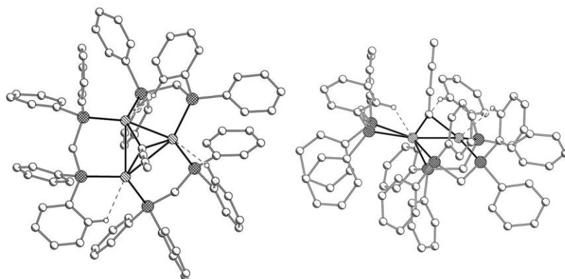
Fig. 7. Projections of the isomorphous [\{M_3(dppm)_3\}(\mu_3-X^1)]^{n+} cations. M = Cu: 1 [6]; M = Ag: 3 (acetone solvate) [6], (no X^2 group).
