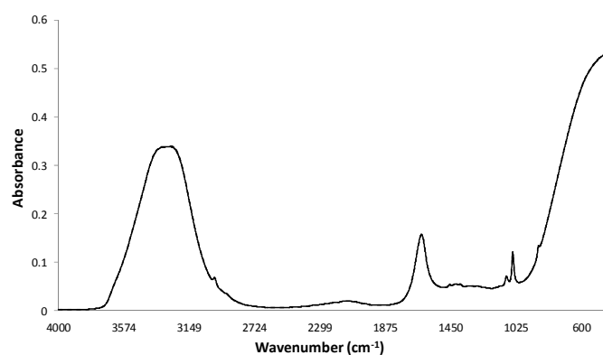
Figure 1. Mean ATR-MIR spectra ( 4000\text{--}400\text{ cm}^{-1} ) obtained from (degassed) French and Australian sparkling wine samples ( n = 45 ).
