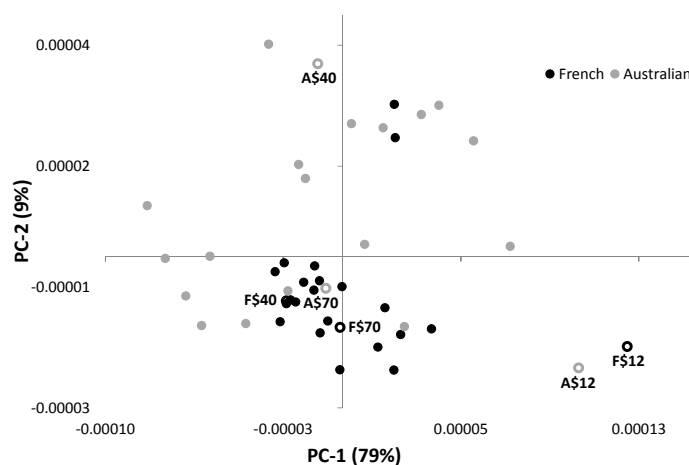
Figure 2. PCA plot generated from the MIR fingerprints ( 1500\text{--}900\text{ cm}^{-1} ) of sparkling wines.
