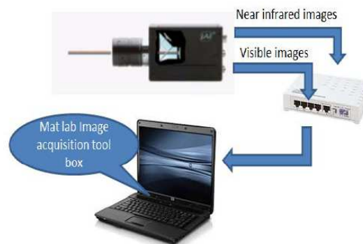
Fig. 6. Equipment set up of the image acquisition
