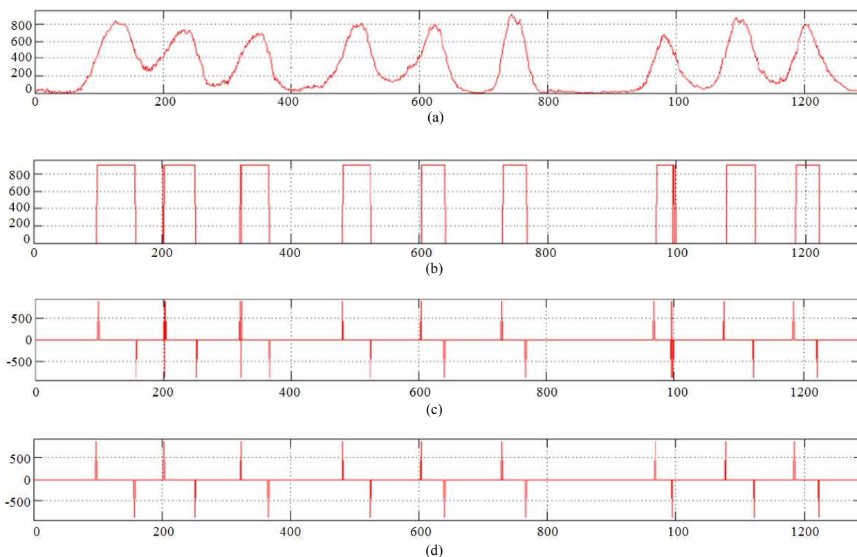
Fig. 14. Detect the dege of the centre part of the crop rows (a) Histogram of column summation S (b) Histogram of Q (After applying the threshold T_1 to S) (c) Histogram of Q' (First order derivative of Q) (d) All the edges of the centre part of the crops are detected, false edges are removed
