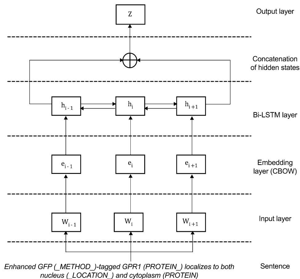
Figure 4. The bi-directional LSTM model to recognize protein subcellular localisation from published literature.
