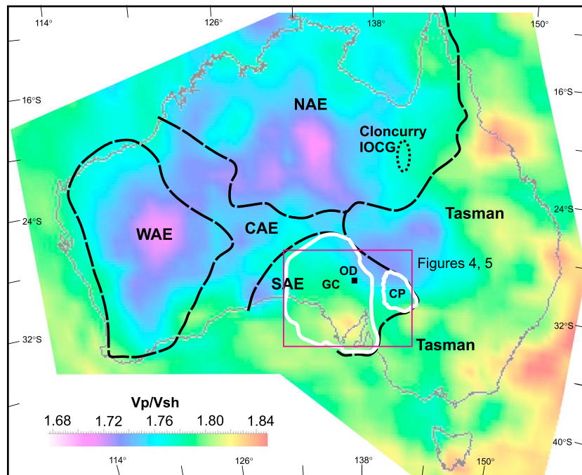
Figure 3. Vp/Vsh map of Australia at ~160 km depth, representing the ratio of P wave ( V_p ) and S wave (horizontal component, V_{sh} ) velocities. Extract from 3-D model (supporting information; see also Appendix A for data sources). Outlines of the Gawler Craton (GC) and Curnamona Province (CP), shown as white lines. Outlines of major Archean-Proterozoic crustal elements (WAE, West Australian element; SAE, South Australian element; NAE, North Australian element) and the Paleozoic Tasman element from Champion (2013). Locations of the Olympic Dam deposit (OD) and the Cloncurry IOCG province are also indicated.
