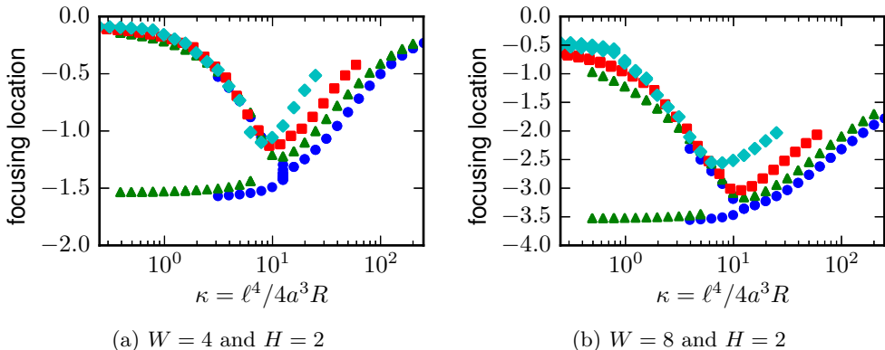
Figure 11: Horizontal location of the (stable) focusing positions of particles versus \kappa = \ell^4/4a^3R for the two rectangular ducts. The particle sizes are a = 0.05 (blue, circles), a = 0.10 (green, triangles), a = 0.15 (red, squares) and a = 0.20 (cyan, diamonds). Note the vertical axis includes only the left half of the duct.
