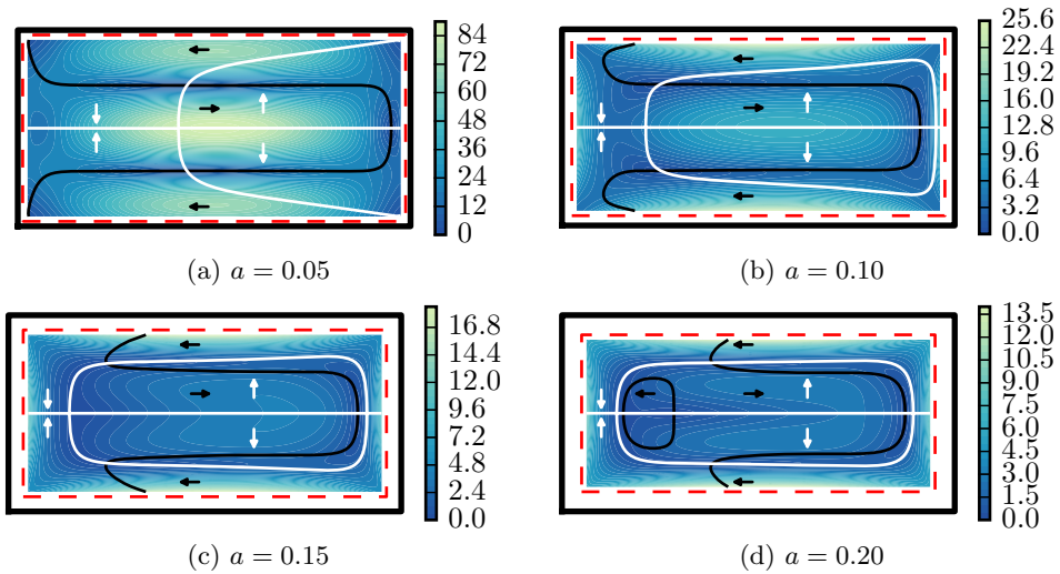
Figure 6: The force F'_p on neutrally buoyant particles at different locations in a curved duct with rectangular cross-section ( W/2 = H = 2 ) and bend radius R = 160 . The colour background shows the magnitude of F'_p . Black and white contours are the zero level set curves of the horizontal and vertical components respectively whereas the arrows indicate the sign of each component in the area bounded by the respective contour. The left wall is on the inside of the bend. The dashed red line shows where the centre of the particle lies when its surface touches the wall.
