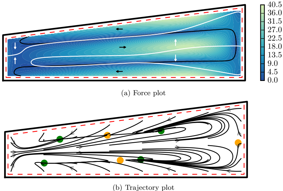
Figure 15: The force F'_p and trajectories of a neutrally buoyant particle having radius a = 0.10 in a curved duct having trapezoidal cross-section ( W = 8 , H_{\text{left}} = 3/2 and H_{\text{right}} = 5/2 ) and bend radius R = 80 . Interpretation of the two plots is the same as in Figures 12 and 13 respectively. Many stable equilibria can be observed in this case.
