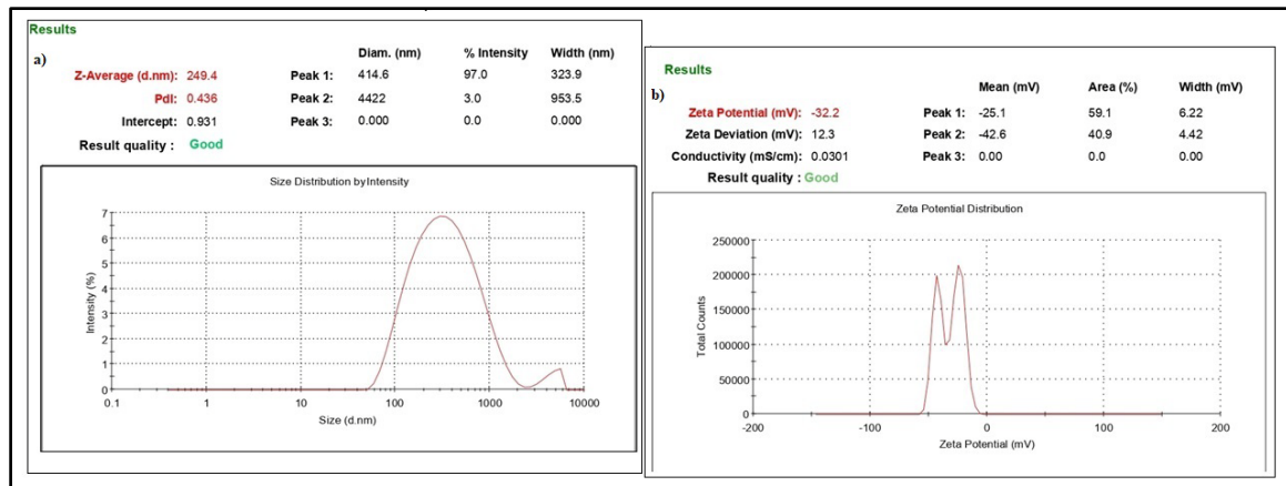
Fig. 9: Particle size (a) and zeta potential (b) of LF9S after 3 mo at accelerated stability condition
