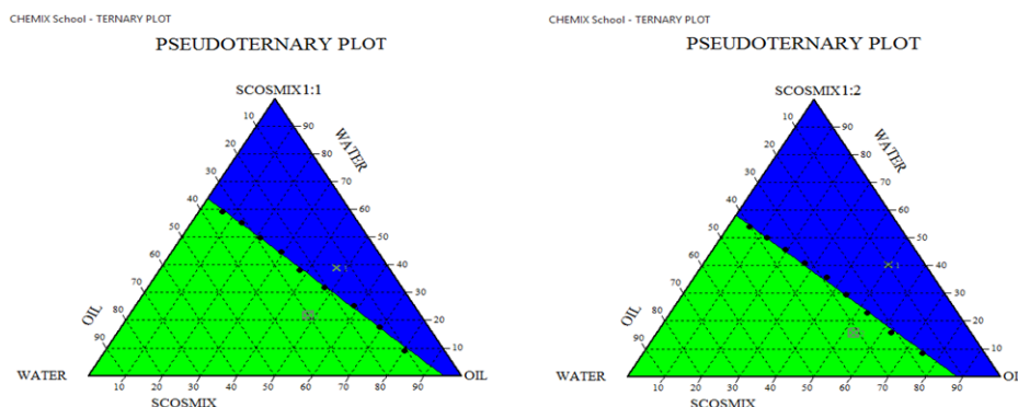
Fig. 2: Represents the ternary phase diagram between linseed oil, tween 80 and PEG 400 (green colored region indicate the self-emulsification region produced by SCOSmix 1:1 ratio (a) and 1:2 ratio (b))
