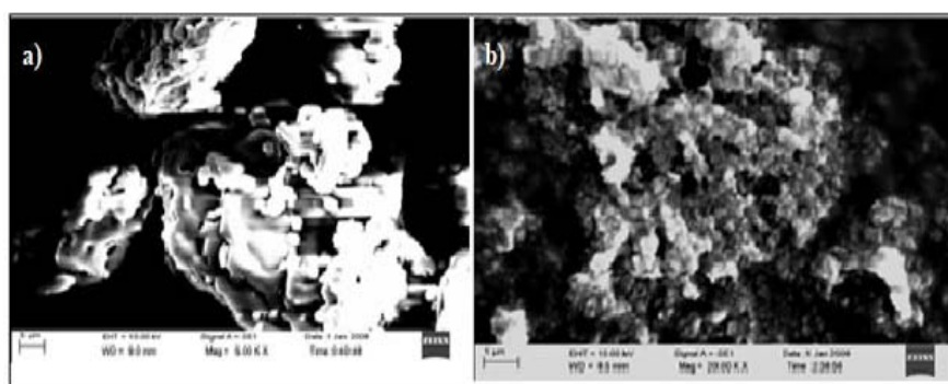
Fig. 7: Scanning electron microscope photograph of nifedipine (a) and LF9S (b)
