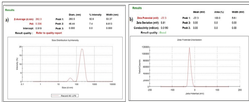
Fig. 4: Particle size (a) and zeta potential (b) of LF9L after 3 mo at accelerated stability condition
