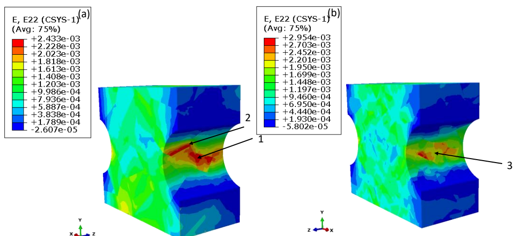
Figure 12. Distribution of the strain component E22 in loading direction for notched specimen for the coarse-grain material (100 grains, (a)) and fine-grained textured material (1000 grains, (b)).
