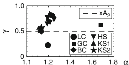
Fig. 10 Parameters \gamma and \alpha for London Clay (LC) [30], Gault Clay (GC) [30], Bangkok Clay (BC), [26] Hostun Sand (HS) [27] and Kenya Sand (KS1, KS2) [8]
