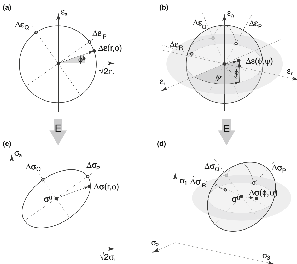
Fig. 13 Isotropic elastic relation \dot{\sigma}(\sigma^0, \dot{\varepsilon}) : a axisymmetric \sigma^0 and co-axisymmetric strain increments \Delta\varepsilon , b diagonal \sigma^0 and coaxial \Delta\varepsilon , c stress response \Delta\sigma for (a) , d stress response \Delta\sigma for (b)
