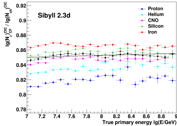
Figure 3: Shower size ratio of Y_{CIC} = \lg(N_{\mu}^{CIC})/\lg(N_{ch}^{CIC}) as a function of true energy, where N_{\mu} and N_{ch} are corrected for attenuation effects in atmosphere using the CIC technique. The dotted line is the separation criteria for heavy and light mass groups.
