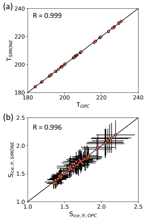
Figure A1. Comparison of the homogeneous freezing onset temperature ( T_{ice} , panel a ) and ice saturation ratio ( S_{ice, fr} , panel b ) derived from the SIMONE and OPC data. The respective Pearson's correlation coefficients are R = 0.999 and R = 0.996 .
