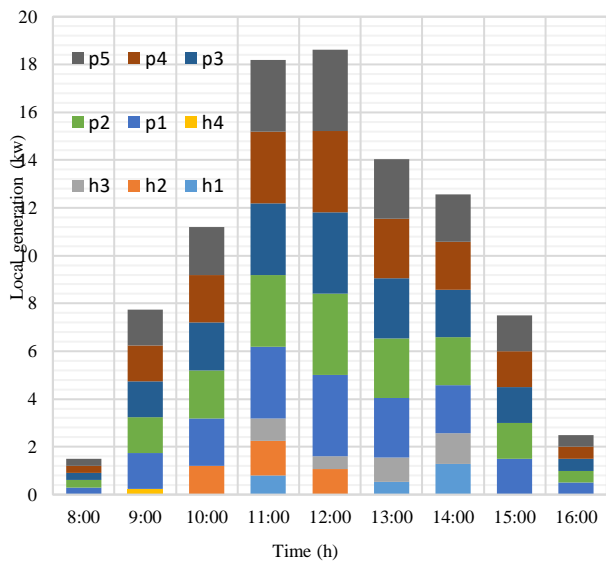
FIGURE 6. The hourly amount of net production for each prosumer
