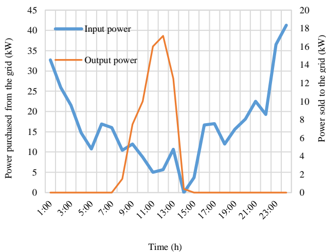
FIGURE 7. The power traded between the local market and the upstream grid
