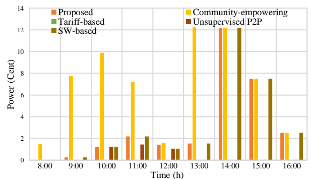
FIGURE 11. Hourly TLT index of households
