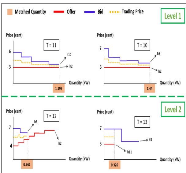
FIGURE 9. Examples of matching of prosumers' offers with consumers' bids considering the proposed model
