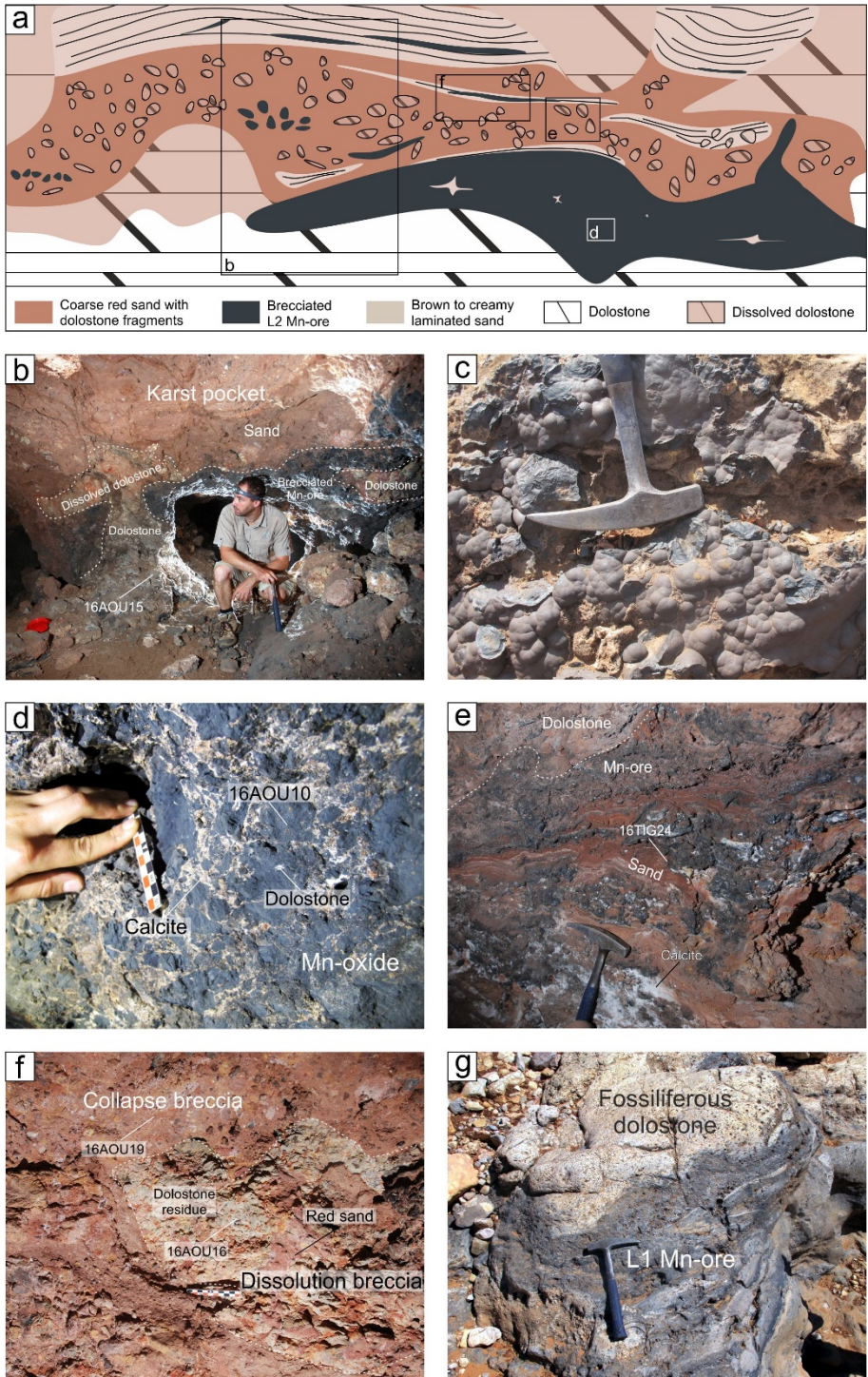
► Fig. 7.31 Field observation of dissolution processes along the Tasdremt district. a. Sketch
