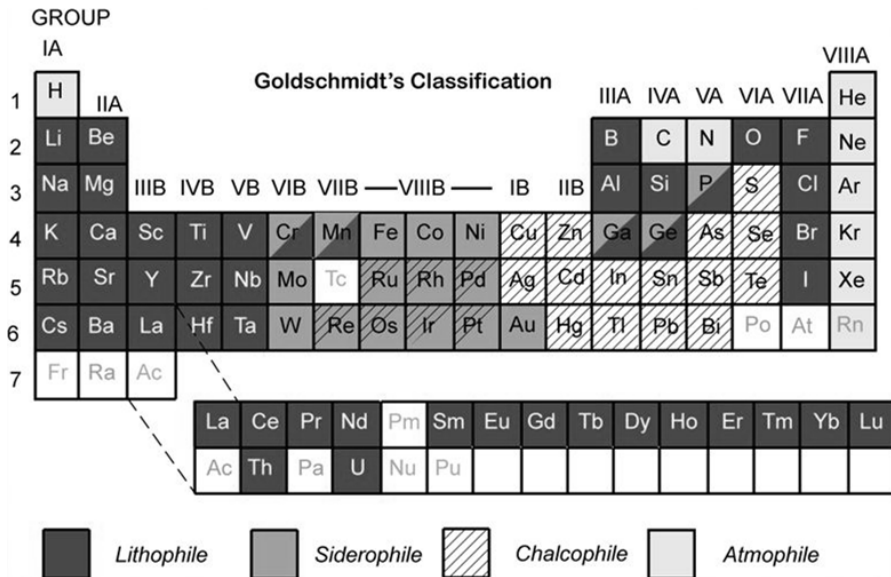
► Fig. 4.7 Goldschmidt's classification of the elements (Winter, 2001).
