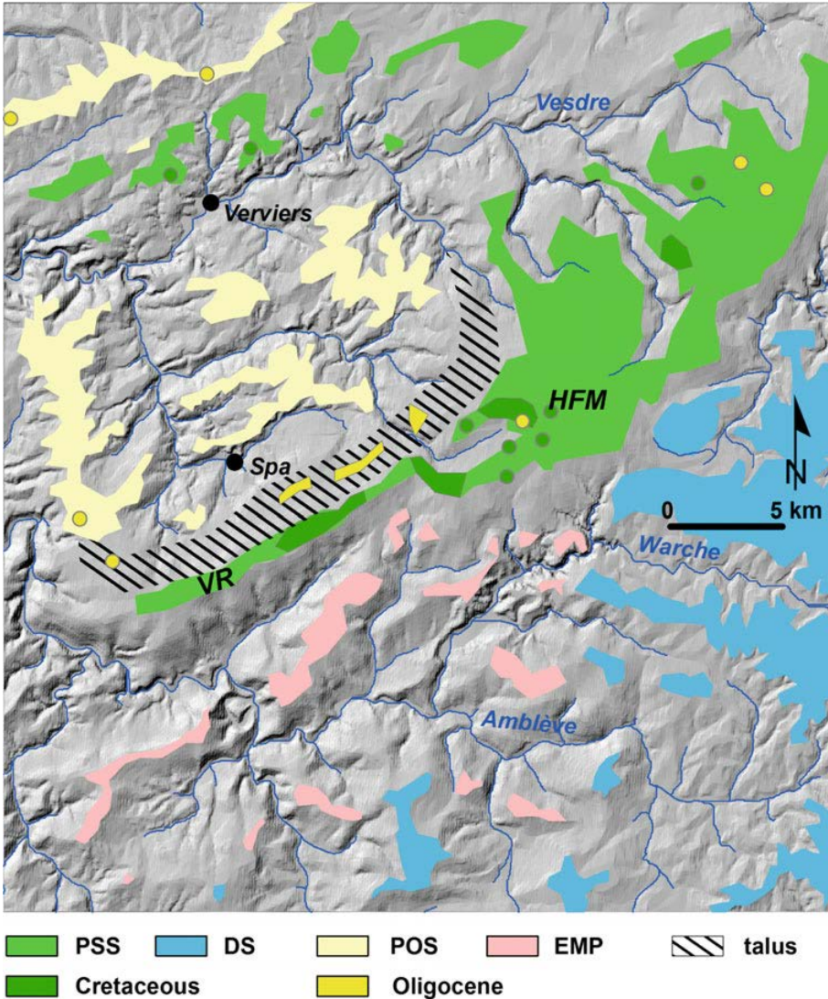
► Fig. 6.11 Map of the erosion surface remnants in the Hautes Fagnes area of NE Ardenne, draped on a hillshade of the SRTM 3'' digital elevation model. All flat interfluvial and broader plateau areas belong to pre-Quaternary topographies of various ages. PSS Pre-Senonian surface. DS Danian surface. POS Pre-Oligocene surface. EMP Early Miocene planation, developed in less resistant Permian conglomerates and Ordovician shales. Talus: ~100-m-high erosional riser between the pre-Senonian/Danian and the pre-Oligocene surfaces as it is preserved since it was carved in the regional topography during the Paleogene.
