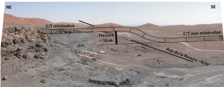
► Fig. 7.42 Offset of the Cenomanian-Turonian level in the Lantenois site. A decametric flexure is observed corresponding to the limit of the mineralization: the southern bottom domain is barren whereas the three mineralized levels are observed in the northern domain. Orientation of the flexure is \sim N70^\circ .
