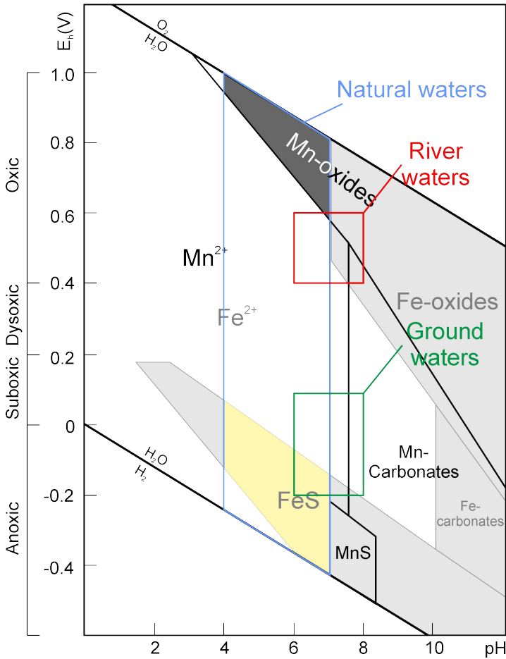
► Fig. 3.9 Synthetic Eh-pH diagram of Mn and Fe (gray shades) at 25 °C and 1 atm with dissolved CO_2 (2,000 mg/l) and sulfate (2,000 mg/ SO_4^{2-} ) showing the main domain where Fe sulfides (yellow field) and Mn oxides (black field) precipitate in natural waters (based on data from Hem, 1963; Glasby, 2006; Roy, 2006; Maynard, 2014). Note that these fields could move slightly toward lower and higher pH values, depending on the Mn^{2+} , HCO_3^- and SO_4^{2-} activities (Hem, 1963).
