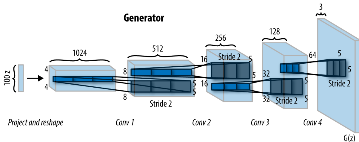
Figure 3.16. Generator network architecture of a 3-D image. Source: [8, 9]
