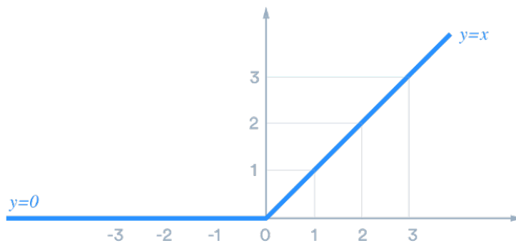
Figure 4.16. ReLU activation function
