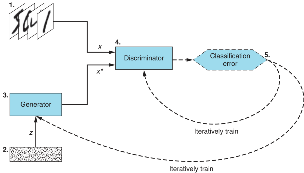
Figure 4.21. GAN training diagram. Source: [13]
