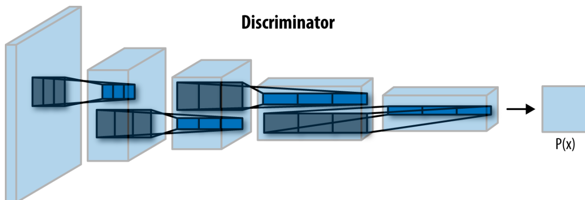
Figure 3.17. Discriminator network architecture of a 3-D image. Source: [8, 9]
