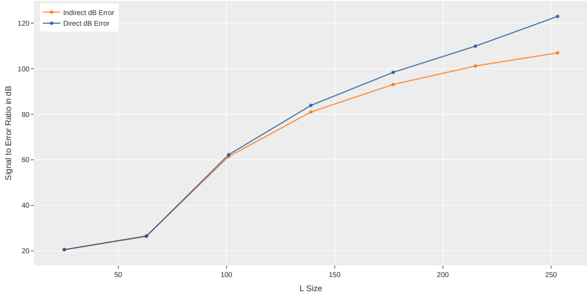
Figure 4.1. SNR x L size for direct and indirect \ell_1 -minimization for 200 random 1D signals
