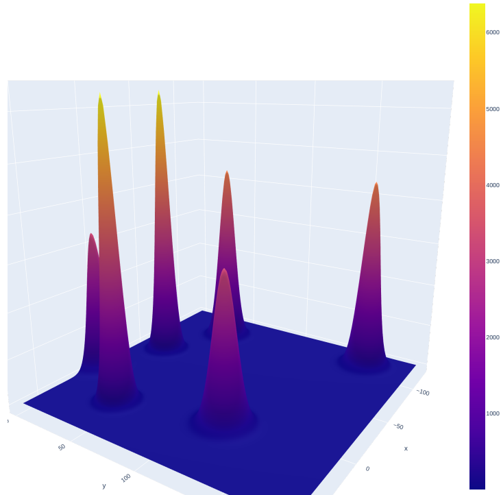
Figure 3.8. Example of Gaussian distributions with four different levels of variances.
