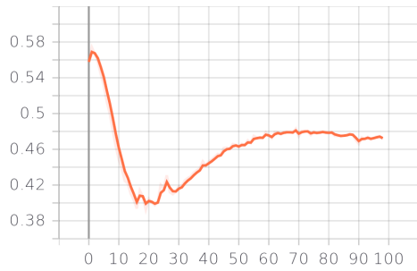
Figure 4.22. Discriminator fake loss over epochs
