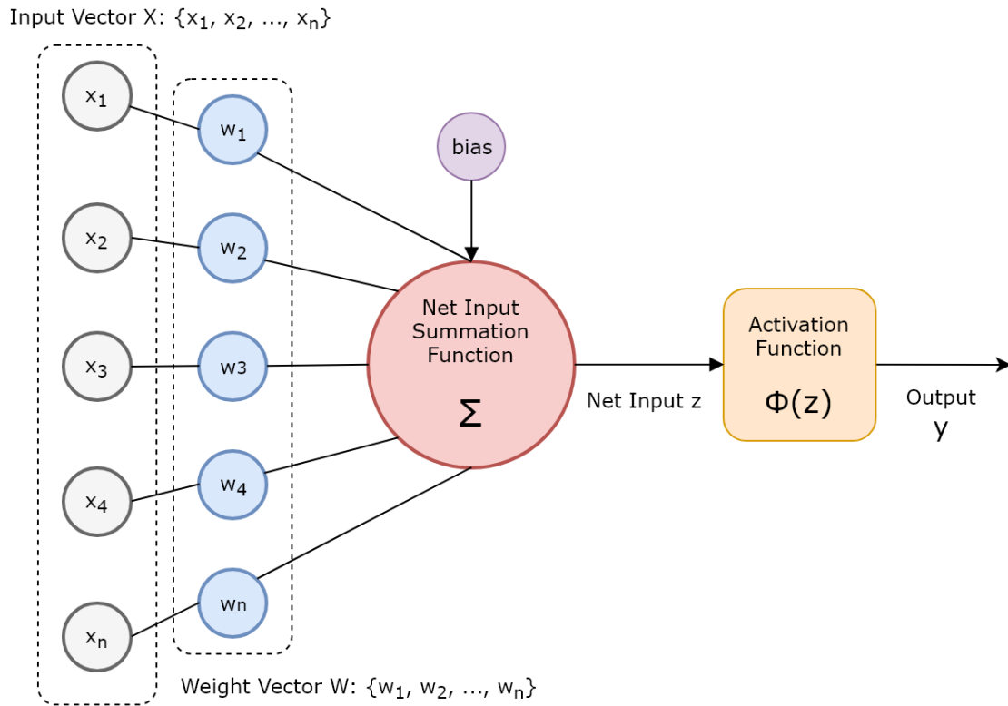
Figure 4.14. Schematic of an Artificial Neuron. Source: [10]
