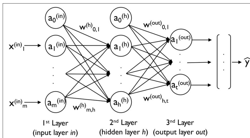
Figure 4.15. ANN Architecture Sample.
