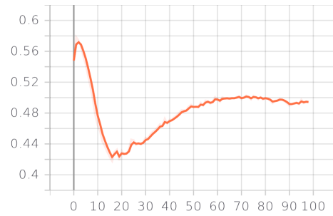
Figure 4.23. Discriminator real loss over epochs
