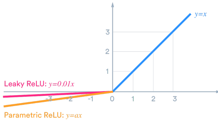
Figure 4.17. Leaky ReLU activation function
