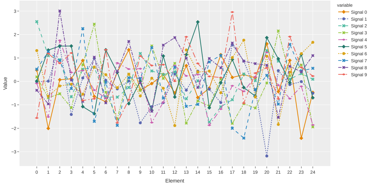
Figure 3.1. First 10 random 1-D signals
