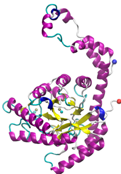
Figure 6. 3D Structure of glucose isomerase from Streptomyces rubiginosus . The crystal structure was solved by Dauter and coworkers; downloaded from rcsb.org (1OAD) [145,199] The structure was visualized using VMD. The N- and C-termini are shown as red and blue spheres respectively while the manganese ions are shown in tan and the magnesium ions shown in cyan. The structure represents one monomer of a homodimer.
