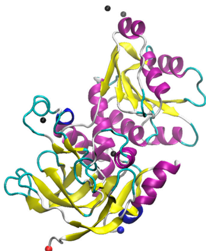
Figure 5. 3D Structure of alcohol dehydrogenase from Saccharomyces cerevisiae . The crystal structure was solved by Ramaswamy and coworkers; downloaded from rcsb.org (5ENV) ([145,193]. The structure was visualized using VMD. The N- and C-termini are shown as red and blue spheres respectively while the zinc ions are shown in black. The structure represents one monomer of a homotetramer.
