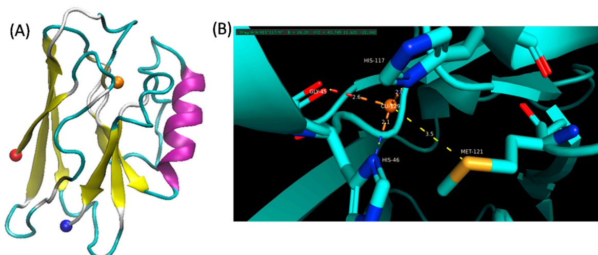
Figure 3. Structure of azurin from Pseudomonas aeruginosa . The crystal structure was solved by Adman and Jensen; downloaded from rcsb.org (1AZU ([182]) [145]) The structure was visualized using VMD. (A) 3D structure of azurin. The N- and C-termini are shown as red and blue spheres respectively while the copper is shown in orange (partially occluded in the structure). (B) Structural geometry of the copper shown in orange and chelating residues highlighted.
