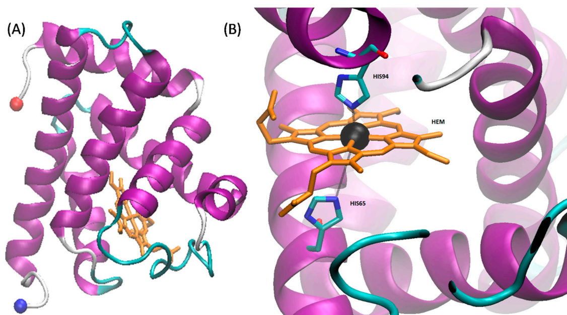
Figure 2. Structure of myoglobin from cardiac muscle of Equus caballus . The crystal structure was solved by Brayer and coworkers; downloaded from rcsb.org (1WLA) [145,173]. The structure was visualized using VMD. (A) 3D structure of myoglobin. The N- and C-termini are shown as red and blue spheres respectively while the heme is shown in orange (partially occluded in the structure). (B) Structural geometry of the heme with the iron shown in black and chelating residues highlighted.
