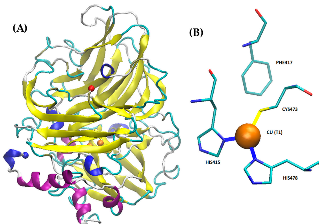
Figure 1. Structure of Laccase from Trametes versicolor . The crystal structure was solved by Choinowski and coworkers; downloaded from rcsb.org (1GYC) ([126,145]). The structure was visualized using Visual Molecular Dynamics (VMD) software. (A) 3D structure of laccase. The N- and C-termini are shown as red and blue spheres, respectively, while the copper ions are shown in orange (partially occluded in the structure). (B) structural geometry of the mono-copper site with chelating residues highlighted.
