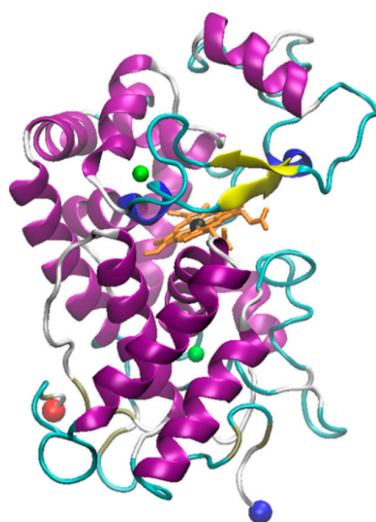
Figure 4. 3D Structure of horseradish peroxidase from Armoracia rusticana . The crystal structure was solved by Hajdu and coworkers; downloaded from rcsb.org (1W4Y) [145,186]. The structure was visualized using VMD. The N- and C-termini are shown as red and blue spheres respectively while the calcium ions are shown in green, the heme in orange and the heme-iron in black.
