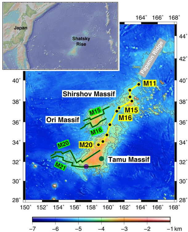
Figure 1. Seafloor depths at Shatsky Rise. (Inset) Setting of Shatsky Rise in the western Pacific Ocean. Figure was made with GeoMapApp ( www.geomapapp.org ), with seafloor depth data from Ryan et al. (2009). (Main panel) The northwestward migration of the Pacific-Izanagi-Farallon triple junction is shown by black-filled yellow dots, accompanied by the magnetic age at which the triple junction occupied each location. Isochrons bracketing the time of formation of Tamu and Ori massifs, which were extracted from Huang et al. (2018) and Sager et al. (2019), are highlighted in green. Locations of drill sites U1347 and 1213 are indicated with green and purple dots, respectively. Seafloor depths are from Smith and Sandwell (1997).
