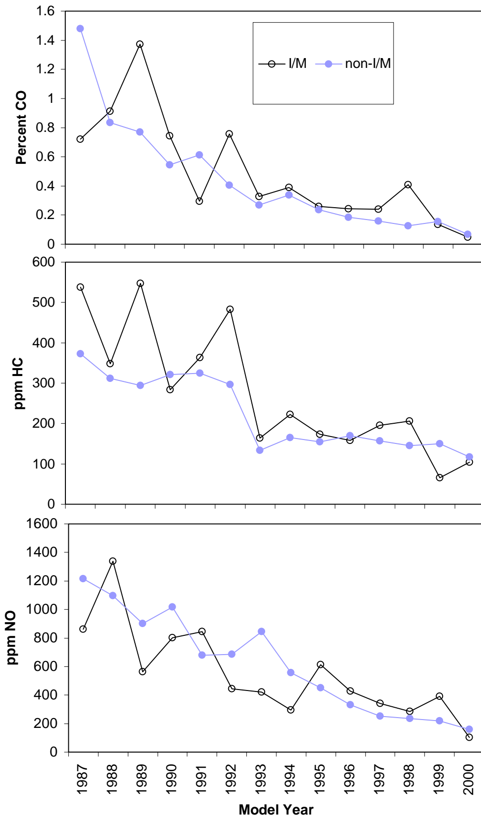
Figure 8. Average emissions as a function of model year of vehicles with IM240 records in 1998, 1999 or 2000 and those with no Colorado IM240 records in the past three years.
