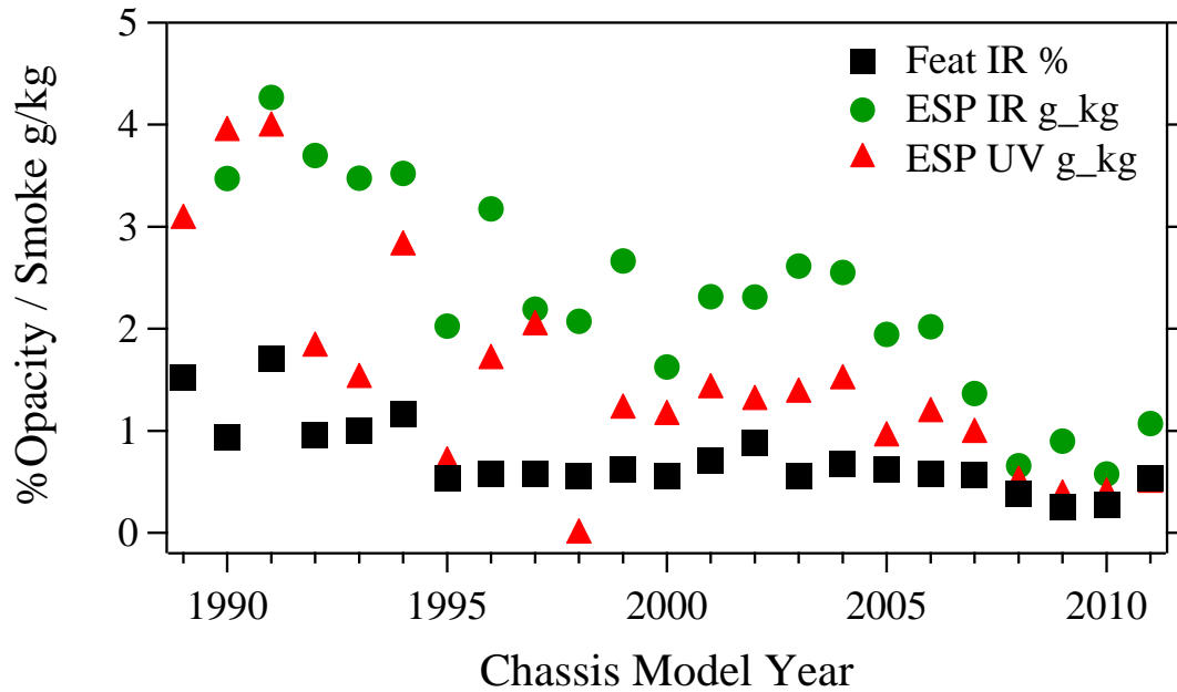
Figure 11. Combined smoke measurements of Peralta and the Port of Los Angeles as a function of chassis model year for the two remote sensing systems. The FEAT reports a % Opacity from the infrared and the ESP system reports smoke (g/kg) in the infrared and the ultraviolet. Model years dating before 1989 are removed because of low sample sizes and high noise.
