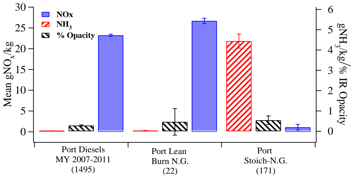
Figure 13. Bar chart of mean emissions of NO x , ammonia and opacity by type of fuel burned and engine type from HDDVs at the Port. Numbers in parentheses are sample sizes. Opacity sample sizes are 1448, 20 and 104 for Diesel, Lean NG and Stoich-NG respectively. Error bars are standard error of the mean.
