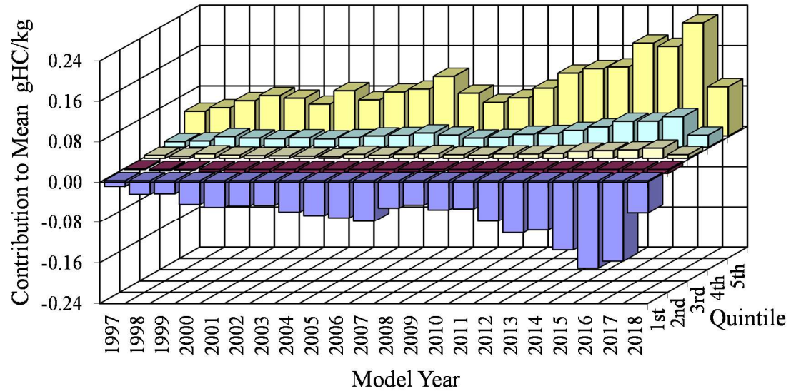
Figure 5. Mean gHC/kg of fuel emissions by model year and quintile (top), fleet distribution (middle) and their product showing the contribution to the mean gHC/kg of fuel emissions by model year and quintile (bottom).
