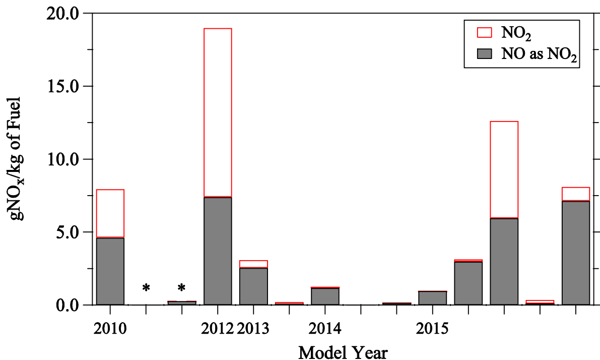
Figure 23. Fuel specific NO x emissions for individual vehicles organized by model year with the model year designation marking the beginning of those model years' measurements. The solid portion of each bar represents the portion of the total NO x emitted as NO in grams of NO 2 and the open portion indicates the amount of NO 2 . The asterisks indicate the same vehicle.
