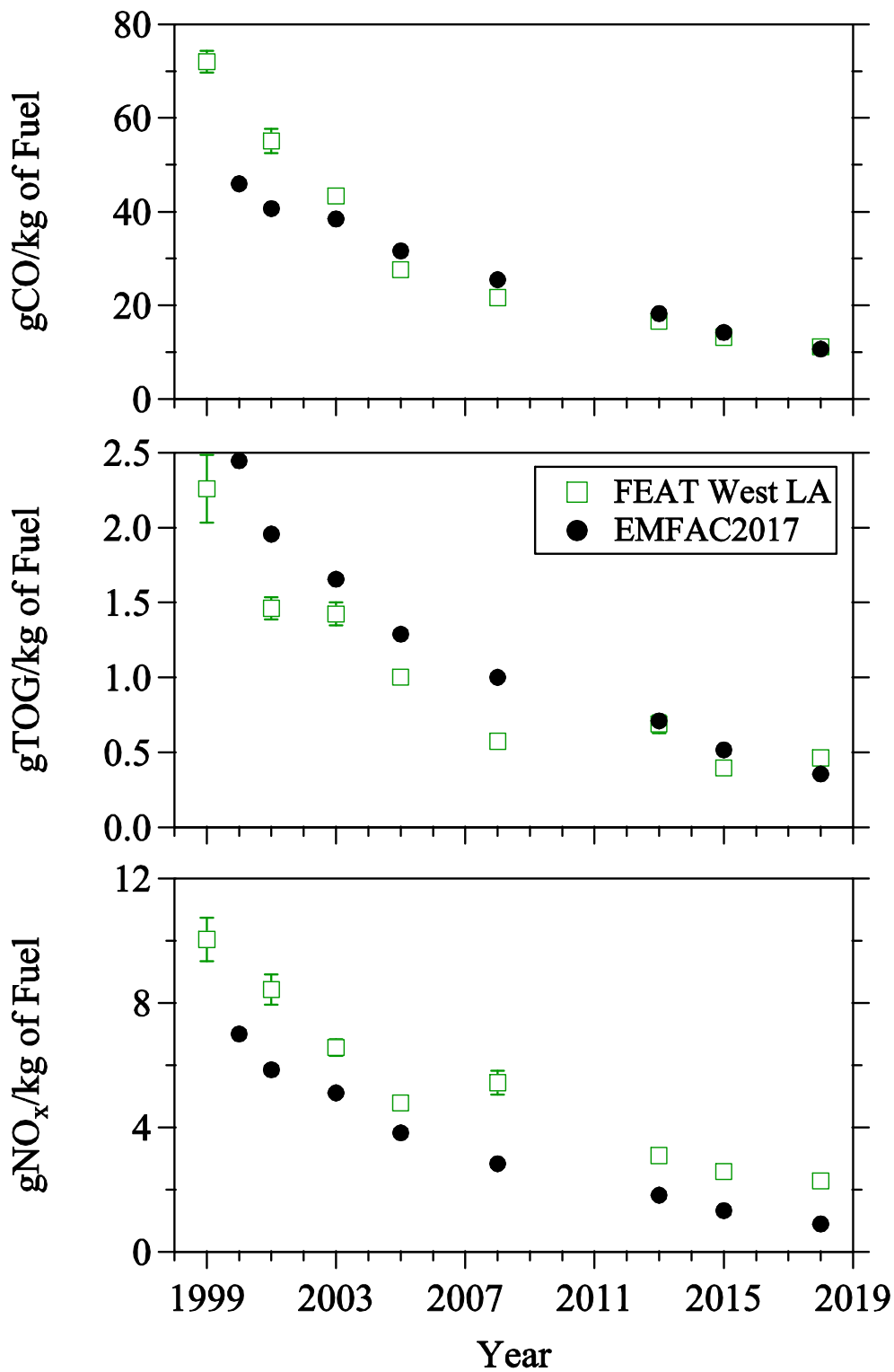
Figure 15. Mean fuel specific CO (top), TOG (middle) and NO x (bottom) emissions comparison between the values measured at the West Los Angeles site for gasoline only vehicles with those predicted by the EMFAC2017 (vehicle types LDA, LDT1, LDT1 and MDV) model. Uncertainties for the measured values are standard error of the mean calculated using the daily values.
