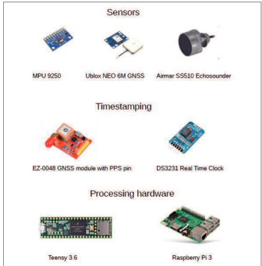
Fig. 1: Main components
