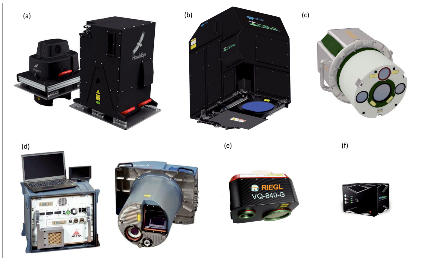
Fig. 2: Examples of airborne laser bathymetry sensors. (a) Chiroptera 4X and HawkEye 4X, (b) CZMIL (Coastal Zone Mapping and Imaging Lidar), (c) VQ-880-GII, (d) Titan Multispectral Lidar, (e) VQ-840-G, (f) ASTRALite edgeLidar
