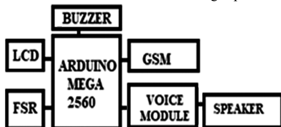
Fig. 1 — Proposed block diagram of Biofeedback device.
