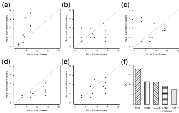
Fig. 4. Accuracy evaluation of the inferred number of clusters. (a–e) Correlations between inferred cluster numbers from SC3, CIDR, Seurat, t-SNE + k -means and SAFE-clustering, respectively, and the true cluster numbers, across the 12 benchmarking datasets. (f) Average deviations between the inferred and the true numbers of clusters, measured by D = \frac{1}{m} \sum_m |k - k_t| , where the number of datasets m equals to 12
