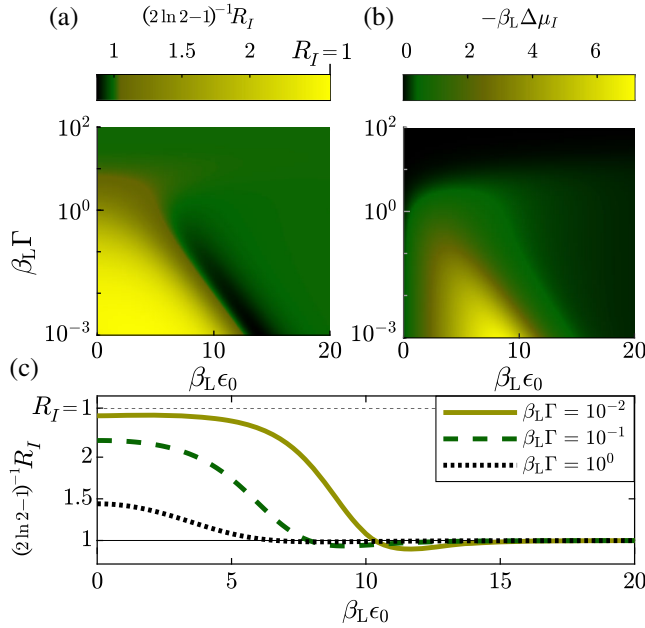
FIG. 2. (a) Charge noise ratio R_I , normalized to the characteristic factor 2 \ln 2 - 1 [see Eq. (7)]. (b) Corresponding charge thermovoltage \Delta \mu_J . (c) Cuts of the density plot in (a) for different values of \Gamma . For all plots, we use D(E) = D_{\text{Lor}}(E) , with D^0 = 10^{-2} , and T_R \ll T_L at fixed, finite T_L .
