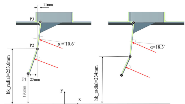
Fig. 7 Scheme for the trigonometrical analysis to obtain the producibility constrain from the operational robot limitation and joint penetration failures
