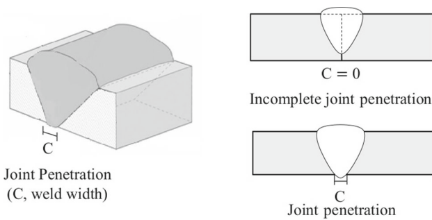
Fig. 8 Producibility failure, joint penetration and weld width, C
