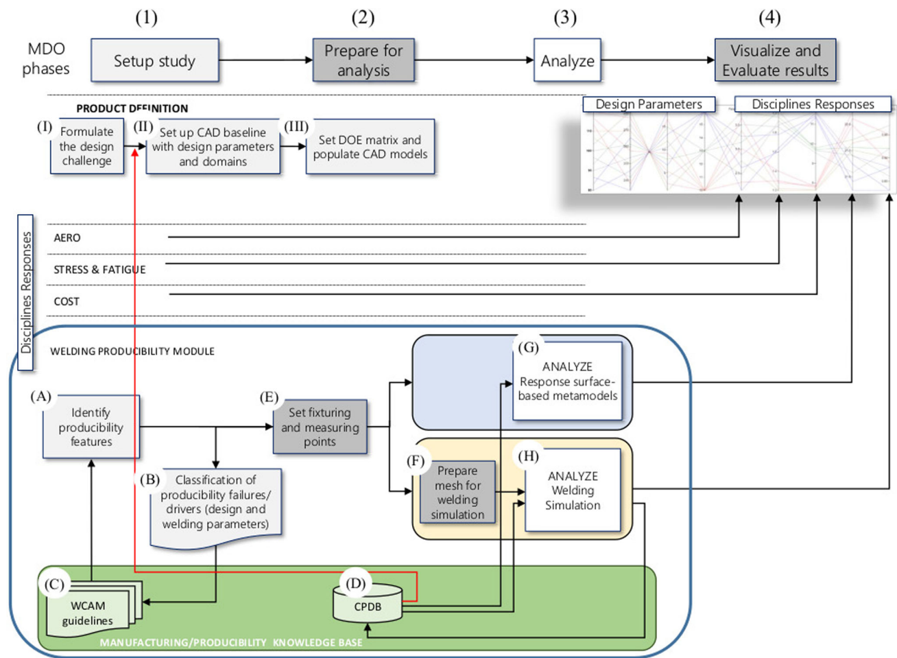
Fig. 2 Automated and interactive MDO welding-producibility assessment module
