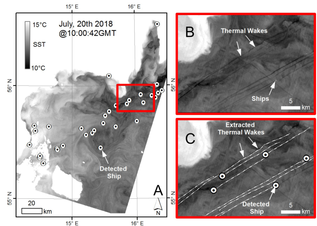
Figure 4. Example of satellite scene with visible thermal wakes in the Bornholm study area, with an illustration of the thermal wake detection process. Panel (a) is the original satellite scene with the detected ships marked as white circles with black dots. The red box marks the zoomed-in area in (b) and (c). In (b), the thermal wakes are visible as darker lines and the ships as small white dots. Panel (c) shows the detected ships and extracted thermal wakes. Landsat-8 image courtesy of the US Geological Survey.
