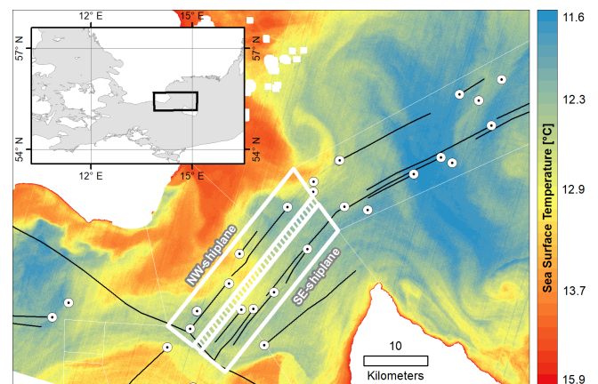
Figure 12. Ships and visible thermal wakes in the Bornholm sound from the analysed satellite scene from 25 May 2014 10:01 LT. White circles with black dots indicate ships with an AIS transmitter present in the area at the time of the satellite passage, and the black lines are the digitalised visible thermal wakes from the satellite scene. White lines indicate the shipping lane area, the bold lines mark the north-west and south-east shipping lanes, and the hatched area is the traffic separation zone. Landsat-8 image courtesy of the US Geological Survey.
