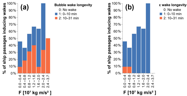
Figure 8. Wake longevity for the bubble wake (a) and dissipation rate of turbulent kinetic energy ( \epsilon ) wake (b), for detected wakes induced by ships passing at zero to three ship widths from the instrument. The x axis shows the force ( F ) of the vessel in newton. Wake temporal longevities < 10 min are shown in blue, and wake longevities 10–31 min are shown in orange.
