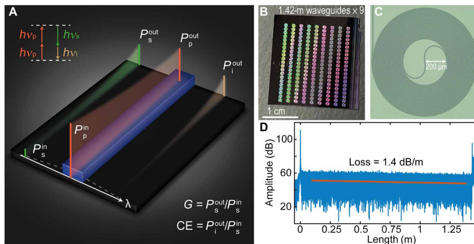
Fig. 1. Schematic illustration of parametric amplification, \text{Si}_3\text{N}_4 chip, and performance characteristics. (A) Schematic illustration of OPAs based on degenerate FWM. The green, orange, and light brown lines represent signal, pump, and idler waves, respectively. (B) Photograph of a representative \text{Si}_3\text{N}_4 chip containing nine waveguides, each with a length of 1.42 m. Photo credit: Z. Ye, Chalmers University of Technology. (C) Optical microscope image of one spiral waveguide unit. (D) OFDR trace of one \text{Si}_3\text{N}_4 waveguide. The measured propagation loss of TE polarization is 1.4 dB/m.
