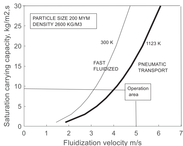
Fig. 5. Accumulative choking velocities according to Bi and Fan (1991), evaluated for 0.2 mm sand-like particles (Replotted from Leckner 2017). The operation area is taken from the Tsinghua state diagram, Yue et al. (2005).
