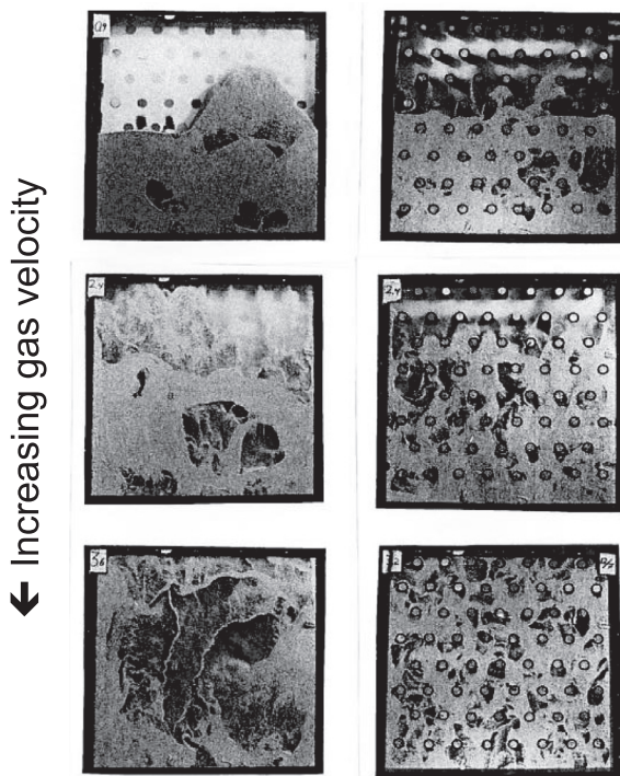
Fig. 3. Images from a cold, two-dimensional bed (dimensions 0.07 \times 0.68 m, and the available height is 3.5 m) operated at velocities u-u_{mf} from 0.24 to 2.0 m/s with (right) and without (left) tubes. The bed particles were sand, size 0.79 mm, Andersson et al. (1989).
