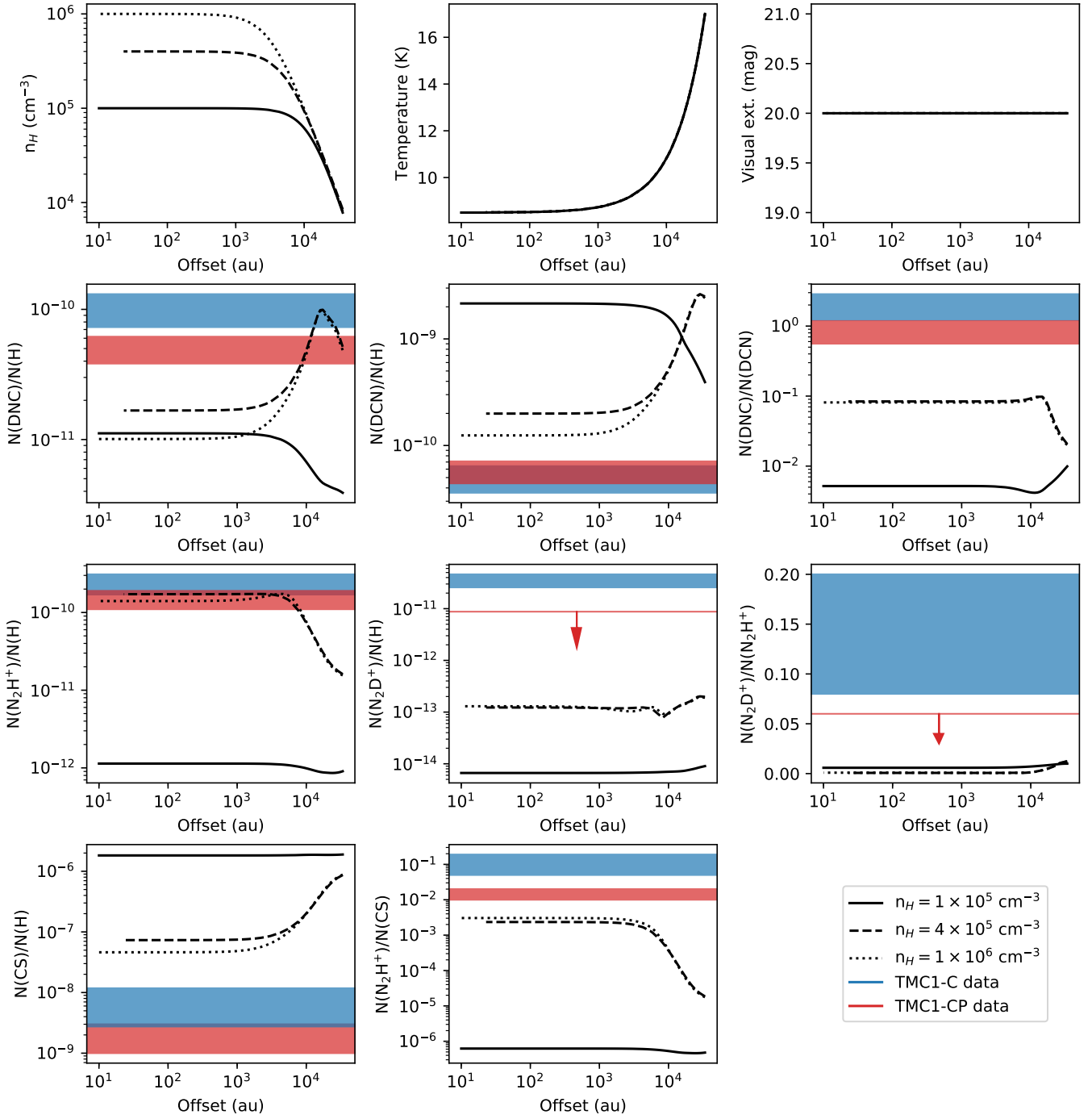
Fig. D.2. Predicted abundances (black) of the different BES4 collapse models with densities 10^5 (solid), 4 \times 10^5 (dashed), and 1 \times 10^6 \text{cm}^{-3} (dotted). The observational data at the center of the starless cores are plotted in blue (TMC 1-C) and red (TMC 1-CP). The arrows indicate upper bounds.
