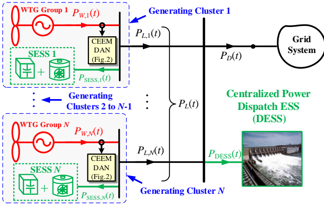
Fig. 1. Conceptual framework of the wide-area wind power generation incorporated with a hierarchical ESS scheme consisting of N distributed power smoothing ESSs (SESSs) and a centralized power dispatch ESS (DESS). The arrows indicate the reference directions of the power flows.
