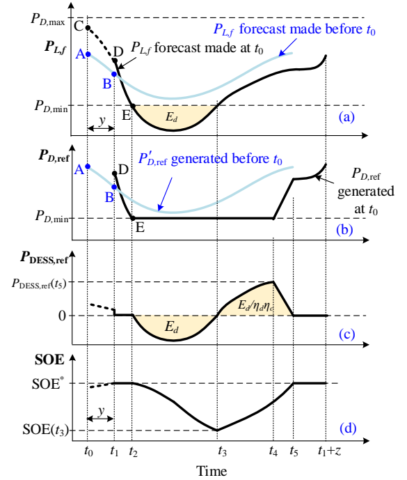
Fig. 6. Example of (a) P_{L,f}(t) determined at and before t_0 , (b) strategized P_{D,\text{ref}}(t) for t_1 \leq t \leq t_1 + z determined at t_0 , (c) strategized P_{\text{DESS,ref}}(t) for t_1 \leq t \leq t_1 + z determined at t_0 , and (d) SOE for t_1 \leq t \leq t_1 + z estimated at t_0 .
