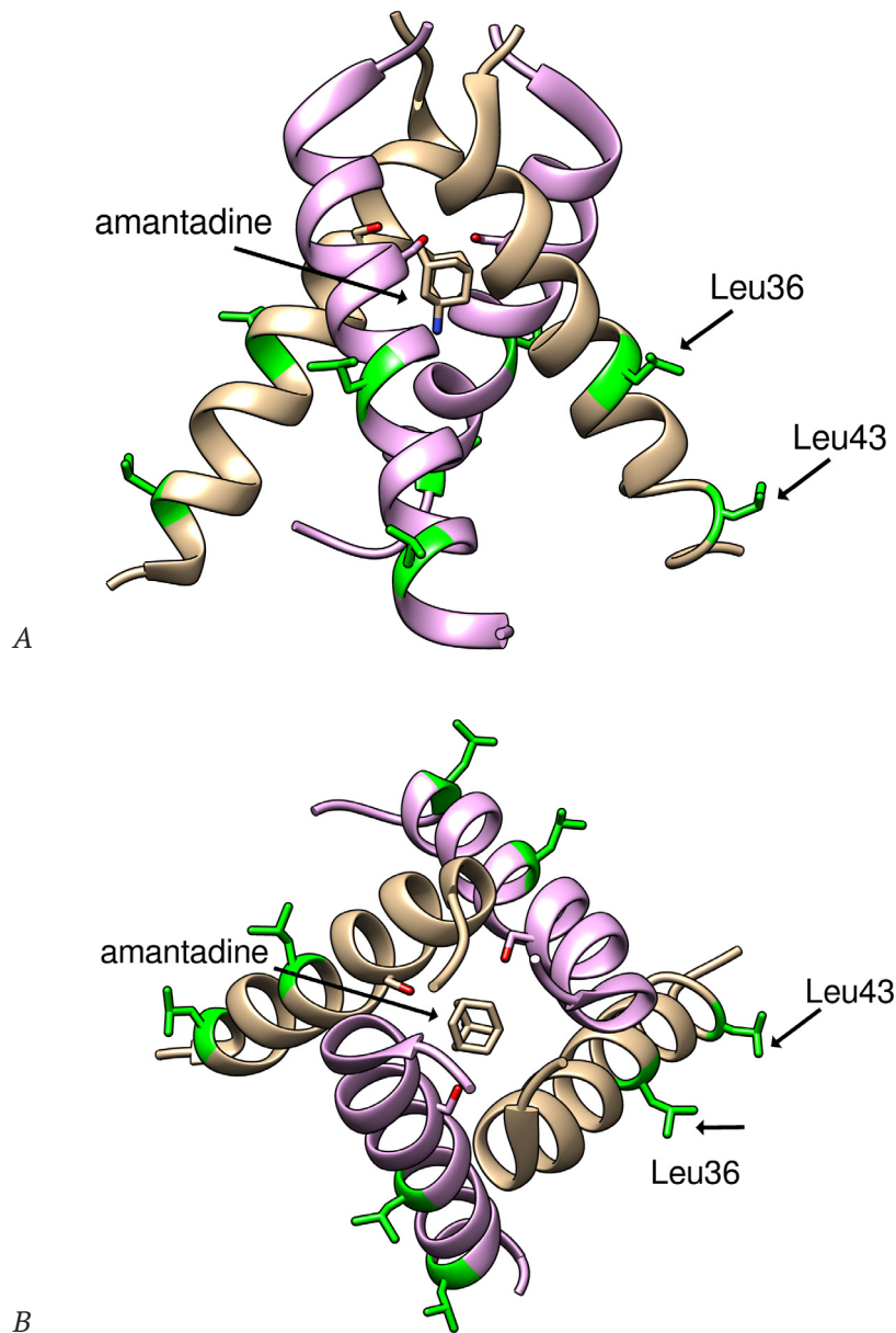
Fig. 6. Structure of the transmembrane domain of influenza virus M2 protein in complex with amantadine.(A) Side view. (B) Top view. Protein Data Bank model 3C9J was visualized using USCf Chimera v.1.10.2 [36]. Mutated amino acids are colored in green.
