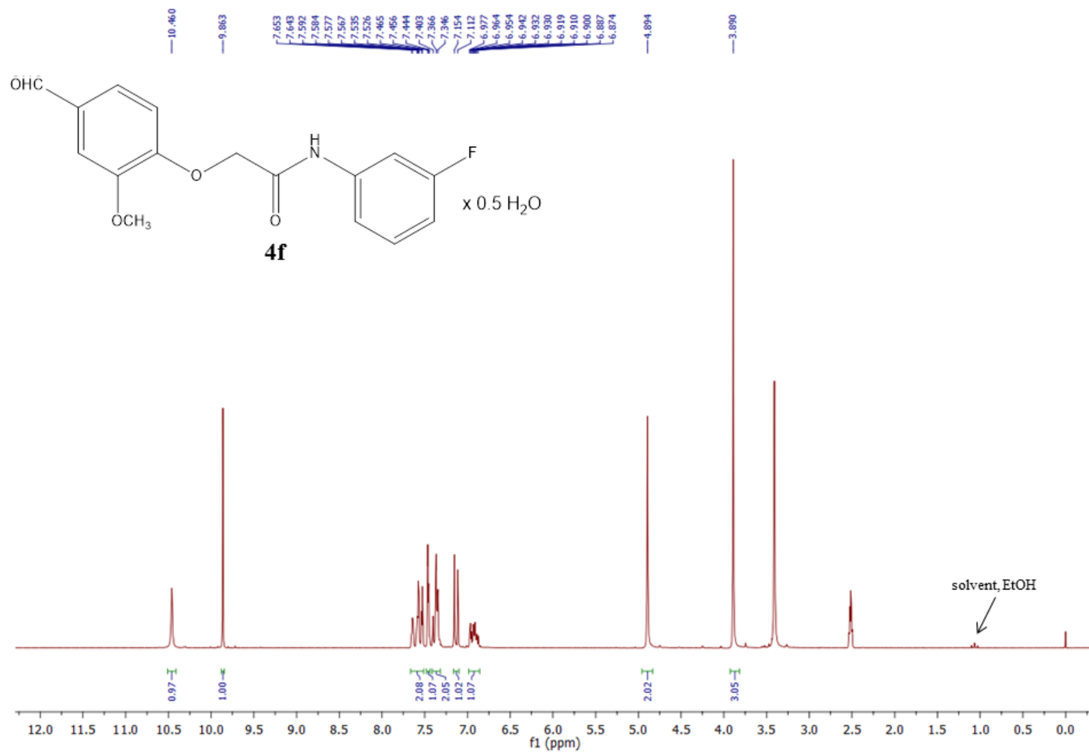
Figure S30. ^1\text{H} NMR spectrum of 4f in DMSO- d_6 (200 MHz).
