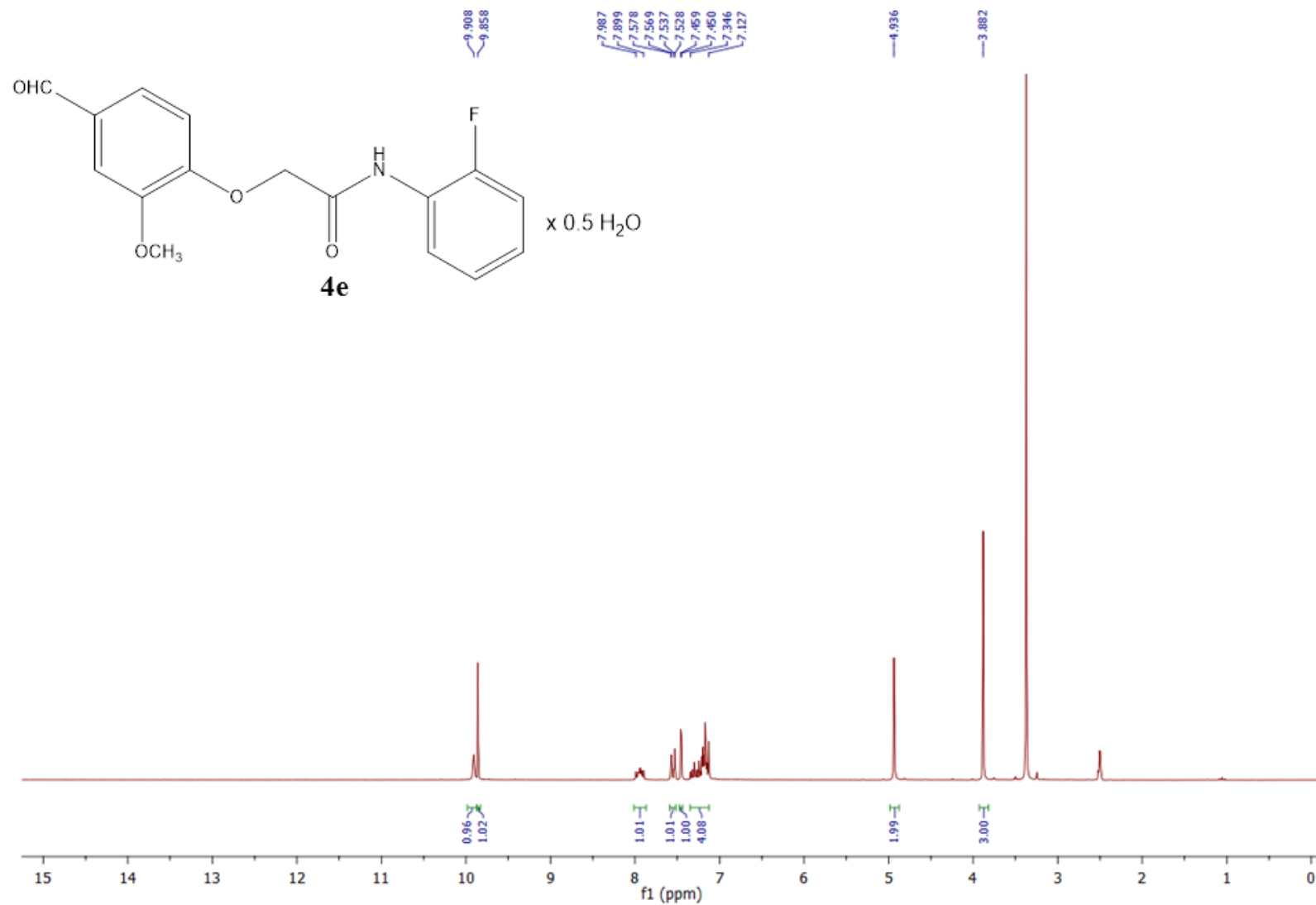
Figure S28. 1 H NMR spectrum of 4e in DMSO-d 6 (200 MHz).
