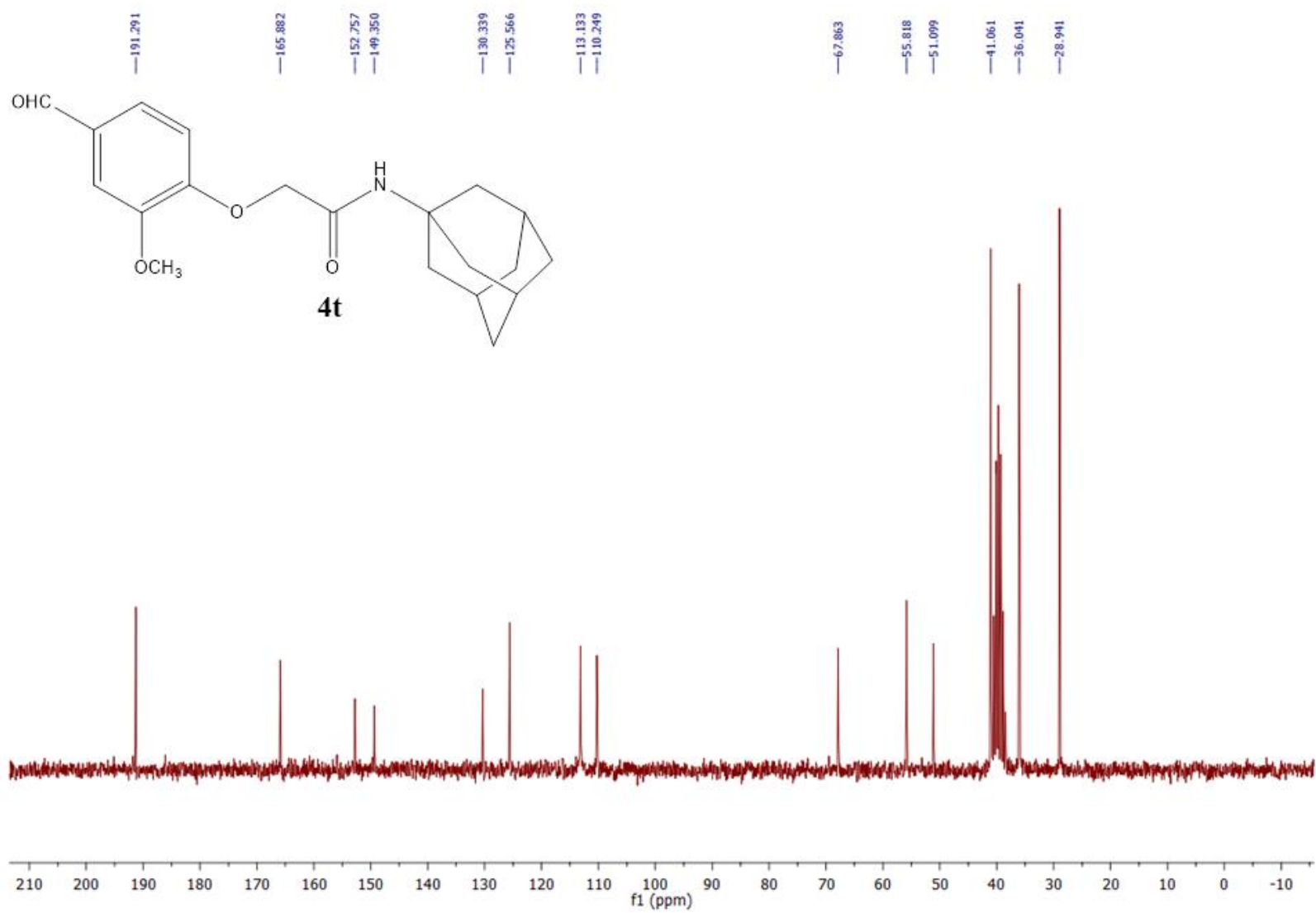
Figure S59. 13 C NMR spectrum of 4t in DMSO-d 6 (50 MHz).
