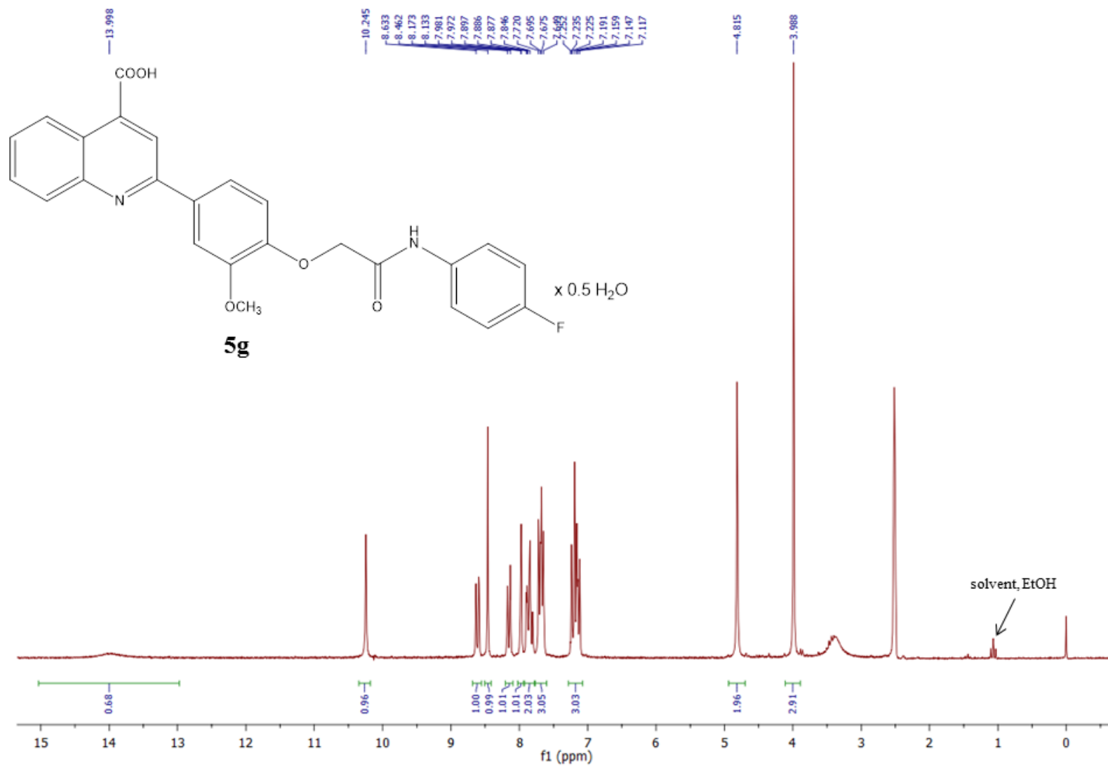
Figure S72. ^1\text{H} NMR spectrum of 5g in \text{DMSO-d}_6 (200 MHz).
