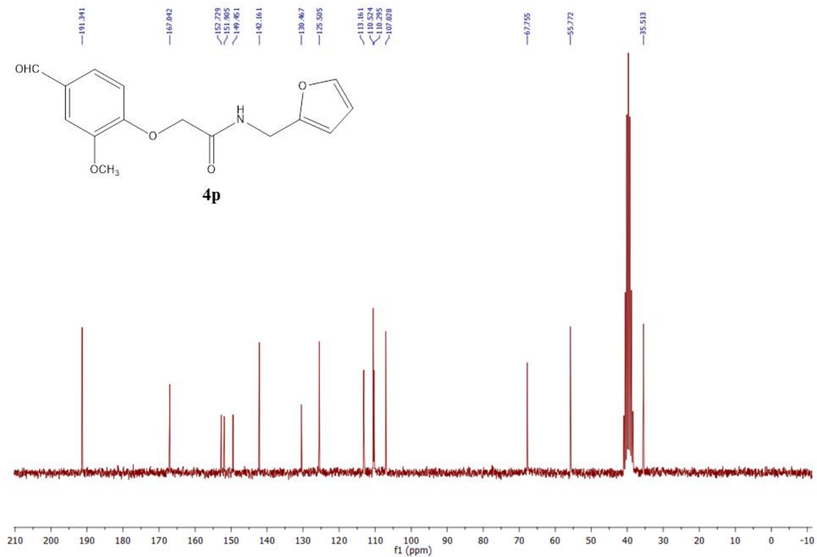
Figure S51. ^{13}\text{C} NMR spectrum of 4p in DMSO- d_6 (50 MHz).
