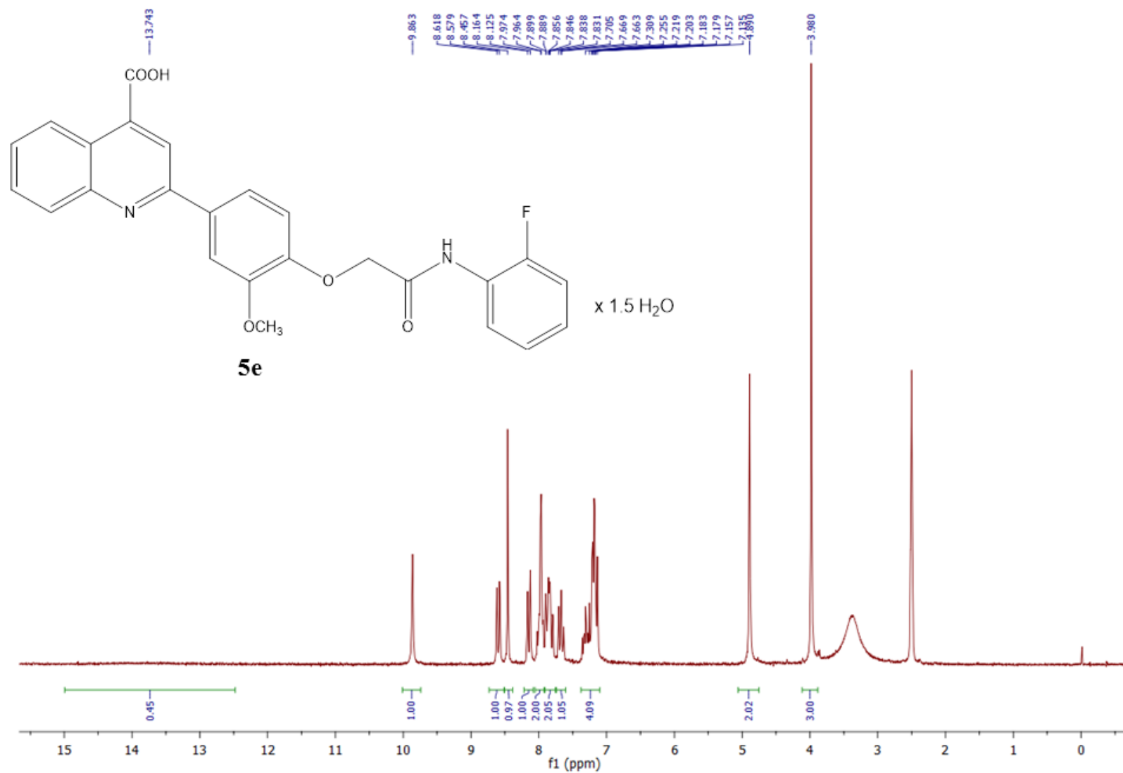
Figure S68. ^1\text{H} NMR spectrum of 5e in \text{DMSO-d}_6 (200 MHz).
