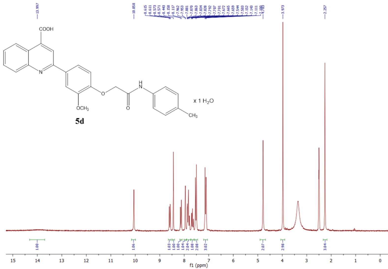
Figure S66. 1 H NMR spectrum of 5d in DMSO-d 6 (200 MHz).
