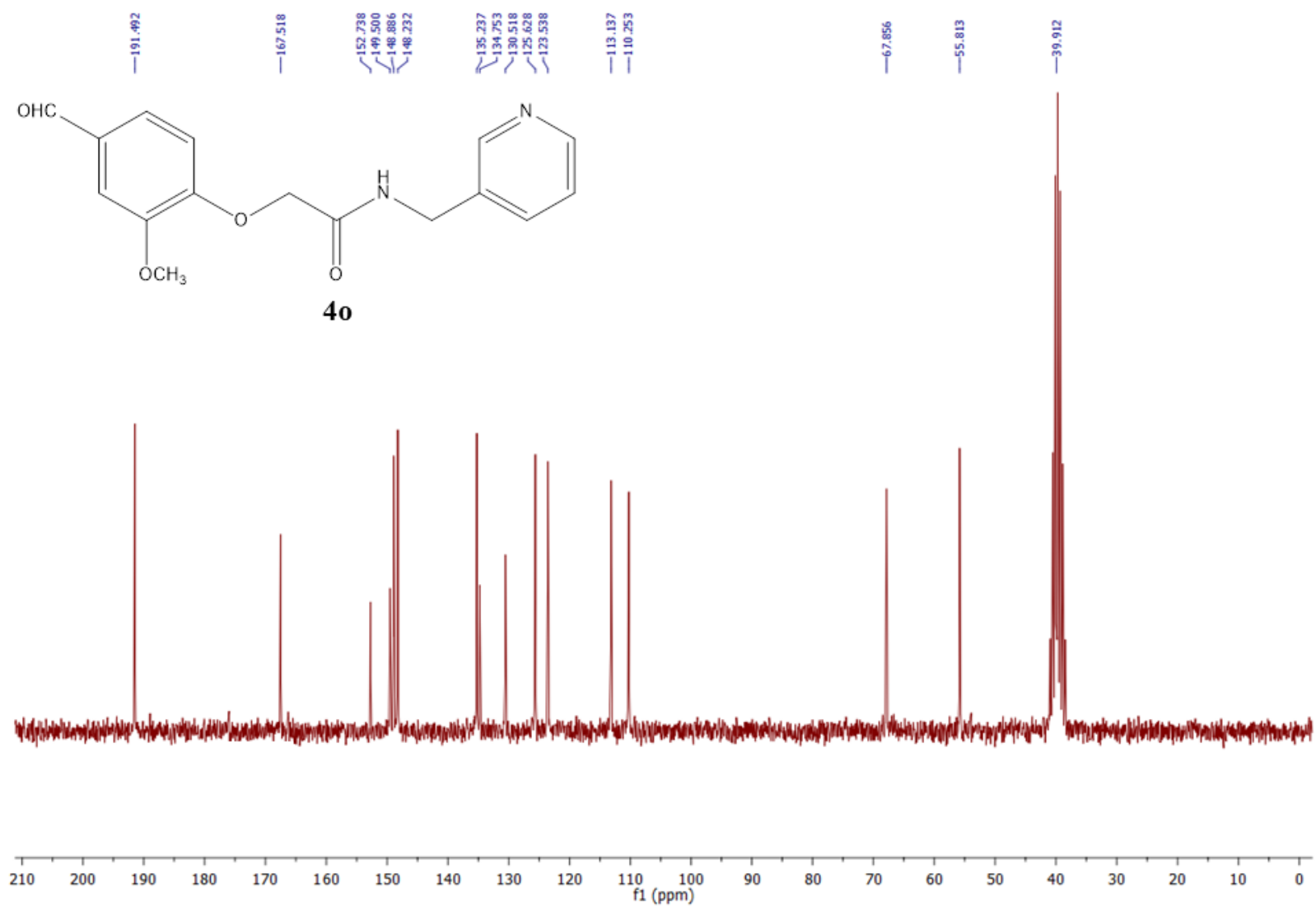
Figure S49. ^{13}\text{C} NMR spectrum of 4o in DMSO- d_6 (50 MHz).
