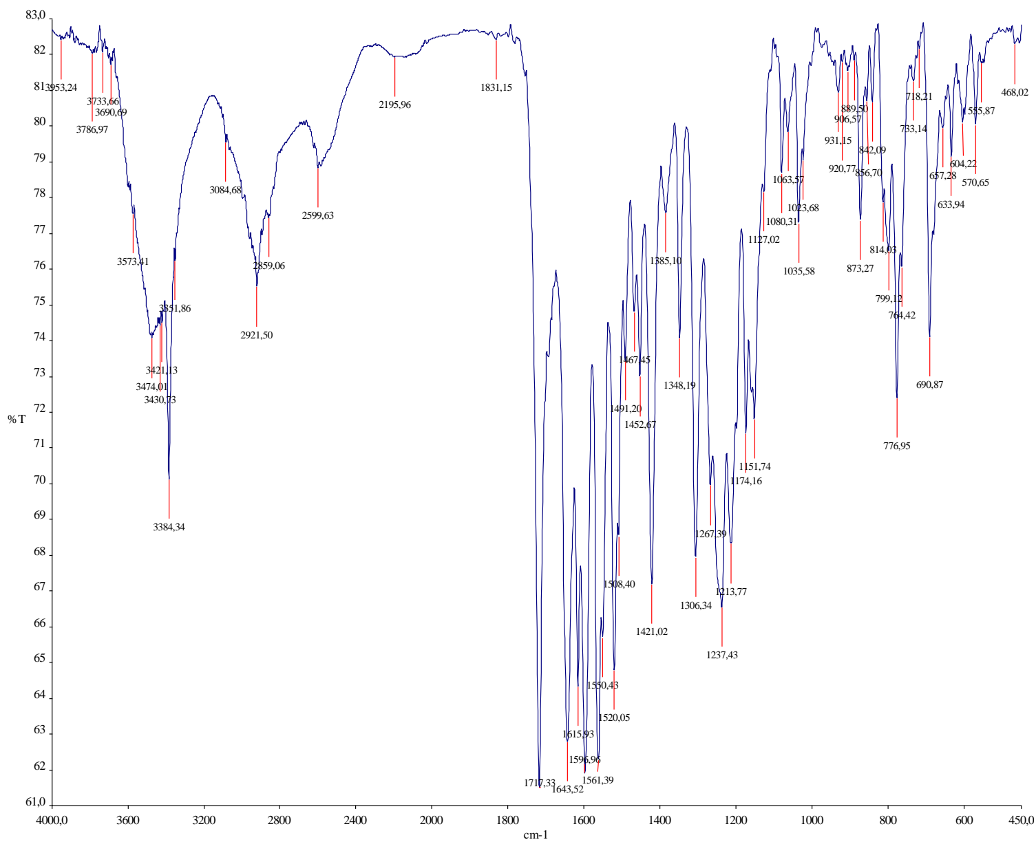
Figure S122. IR spectrum of 5c.
