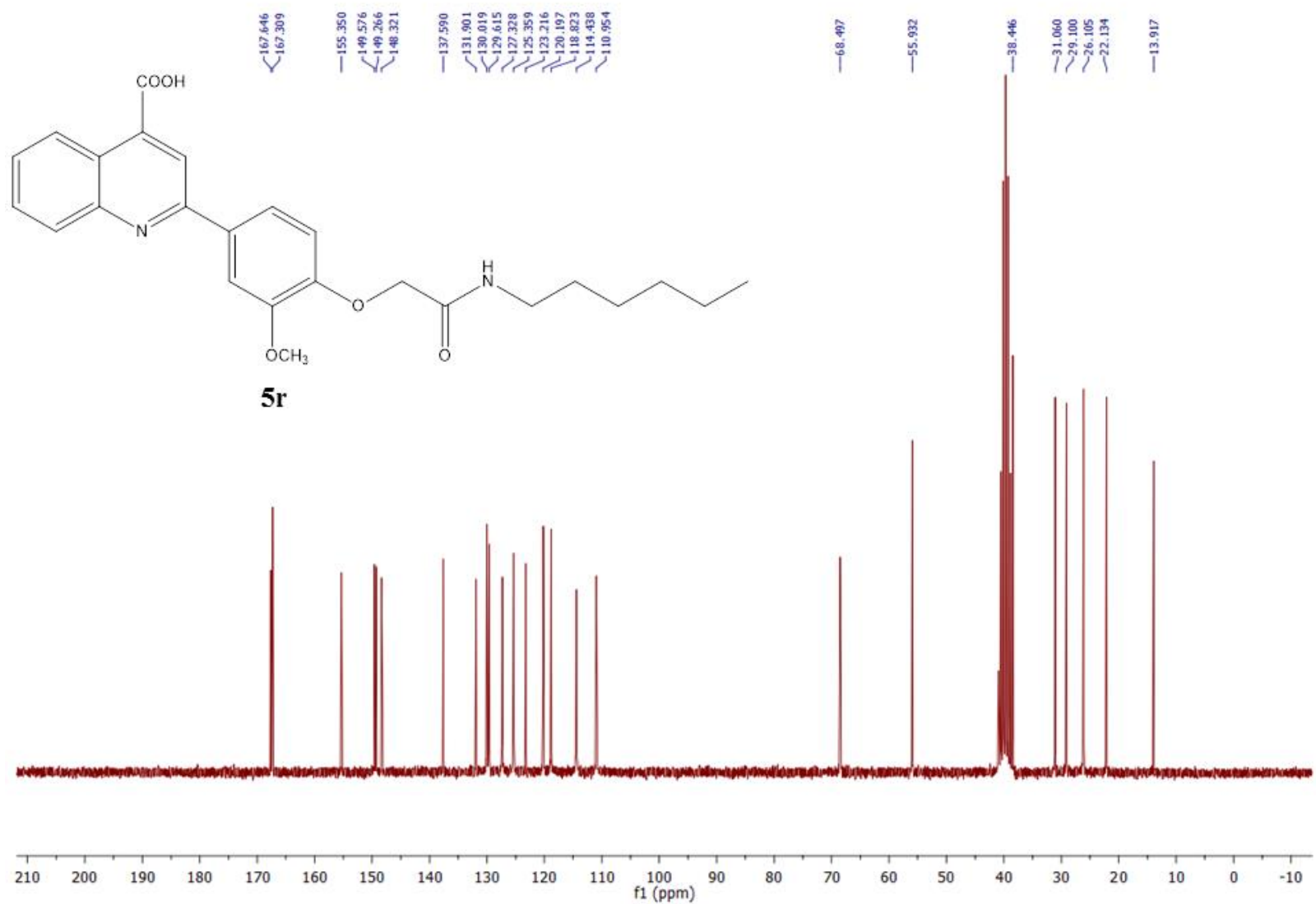
Figure S95. ^{13}\text{C} NMR spectrum of 5r in DMSO- d_6 (50 MHz).
