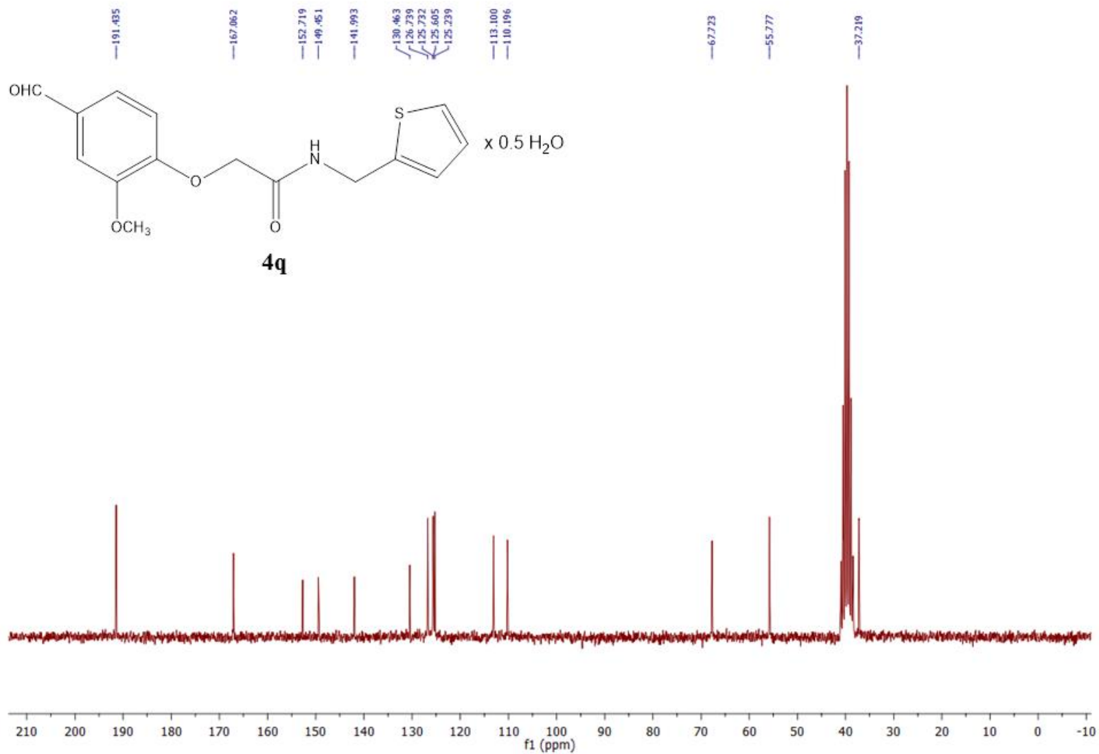
Figure S53. 13 C NMR spectrum of 4q in DMSO-d 6 (50 MHz).
