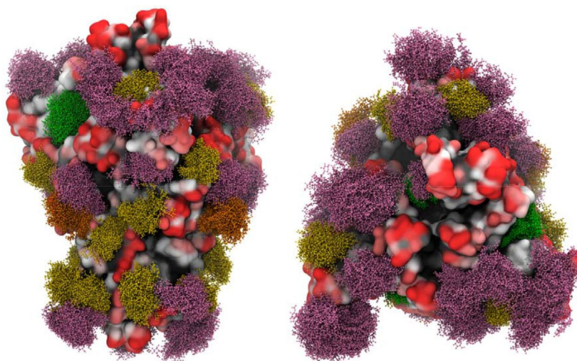
Fig. 15. 3D models of the glycosylated S (spike) protein of SARS-CoV-2. High-mannose structures \text{Man}_9 are depicted in green and \text{Man}_5 in dark yellow. Hybrid N-glycans are shown in orange and complex N-glycans in pink. Figure reproduced from Ref. [321].
