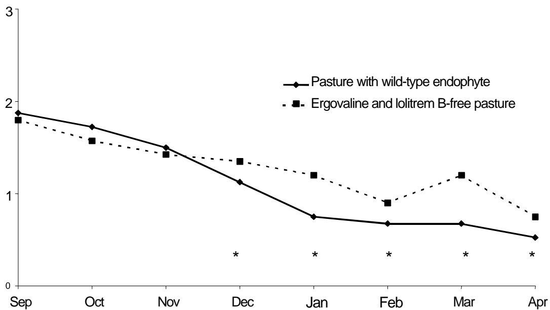
Figure 1 - Dairy milk solids production as affected by endophyte toxins. Reproduced with permission (Blackwell & Keogh 1999).
