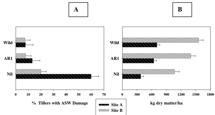
Figure 2 - (A) Effect of the wild-type endophyte (wild), the novel endophyte, AR1, and endophyte-free (Nil) ryegrass on tiller damage by Argentine stem weevil (ASW) larvae at two sites in the North Island of New Zealand, and (B) the associated ryegrass yields after damage had occurred. Extracted with permission from Popay et al (1999).
