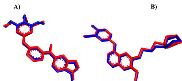
Figure 8. iGEMDOCK validation. (A) Crystal KIM (red) and the docked one (blue) display similar binding orientation in the binding pocket of VEGFR-2 with RMSD 0.4355 Å. (B) Crystal gefitinib (red) with the docked one (blue) are superimposed in EGFR binding cavity with RMSD 0.3462 Å.
