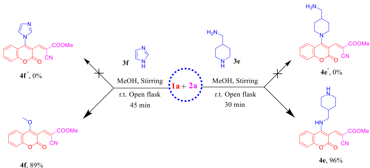
Scheme 2. Synthesis of 4e and 4f .
