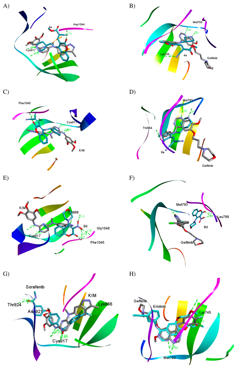
Figure 6. (A, C, E and G) Three-dimensional docking poses of 4e , 8e , 9d , and sorafenib (cyan), respectively, with KIM (grey) within the binding site of VEGFR-2 (PDB ID: 3CJG). (B, D, F and H) Three-dimensional binding modes of 4e , 8e , 9d , and erlotinib (cyan), respectively, with gefitinib (grey) within the active site of EGFR (PDB ID: 4WKQ). H-bonds are denoted by dashed lines in green. All pictures were prepared with Discovery Studio Visualizer Client 2020, and are simple for clarity of presentation.
