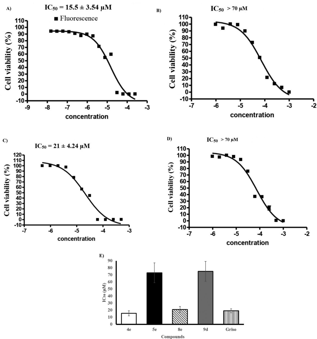
Figure 2. Sigmoidal dose–response against KB-3-1 cell line; (A) 4e , (B) 5e , (C) 8e , (D) 9d , and (E) graph show the IC 50 values of the tested compounds 4e , 5e , 8e , 9d , and (+)-griseofulvin as a positive control.
