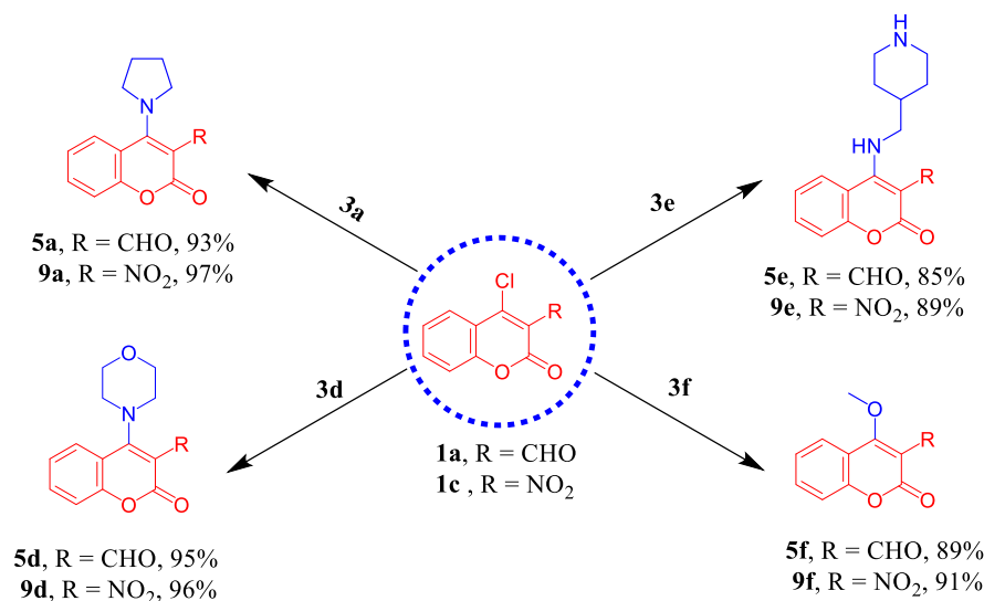
Scheme 6. Previous work by Yang and Vyasamudri groups as well as scope of various cyclic secondary amines for the synthesis of 5a , d-f and 9a,d-f . Reagents and conditions: 1a,c (1.0 mmol, 1.0 equiv), 3a,d-f (1.0 mmol, 1.0 equiv), and \text{Et}_3\text{N} (1 mmol, 1 equiv) in MeOH (2 mL) using open flask at room temperature under stirring conditions, R = CHO, 15 min, R = \text{NO}_2 , 5 min.
