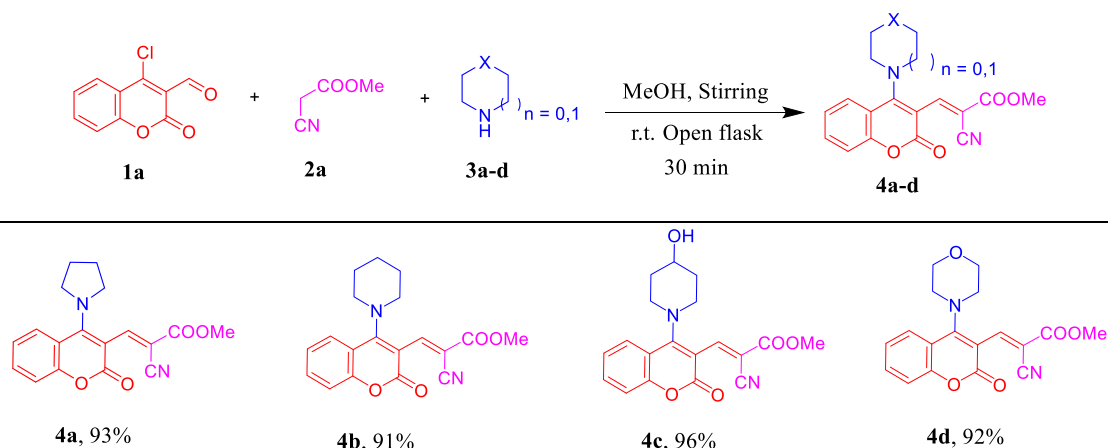
Scheme 1. Scope of various cyclic secondary amines for the synthesis of 4a-d . Reagents and conditions: 1a (1.0 mmol, 1.0 equiv), 2a (1.0 mmol, 1.0 equiv), and 3a-d (2.5 mmol, 2.5 equiv) in MeOH (2 mL) using open flask at room temperature under stirring conditions.
