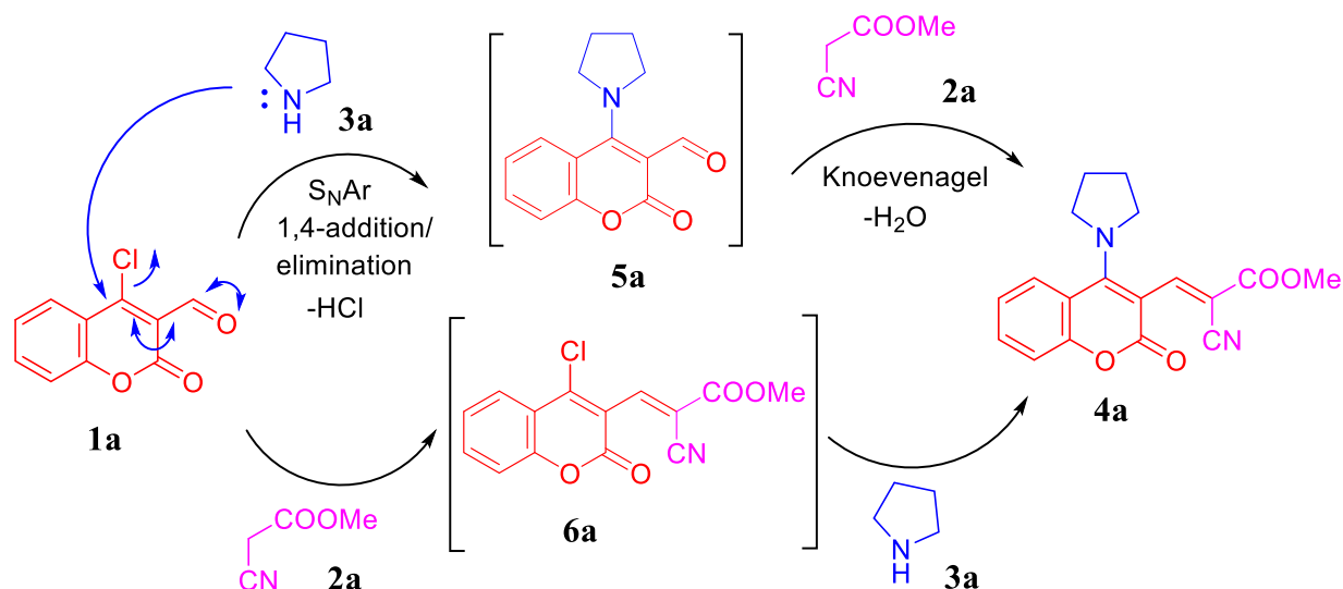
Scheme 4. Plausible reaction mechanism.
