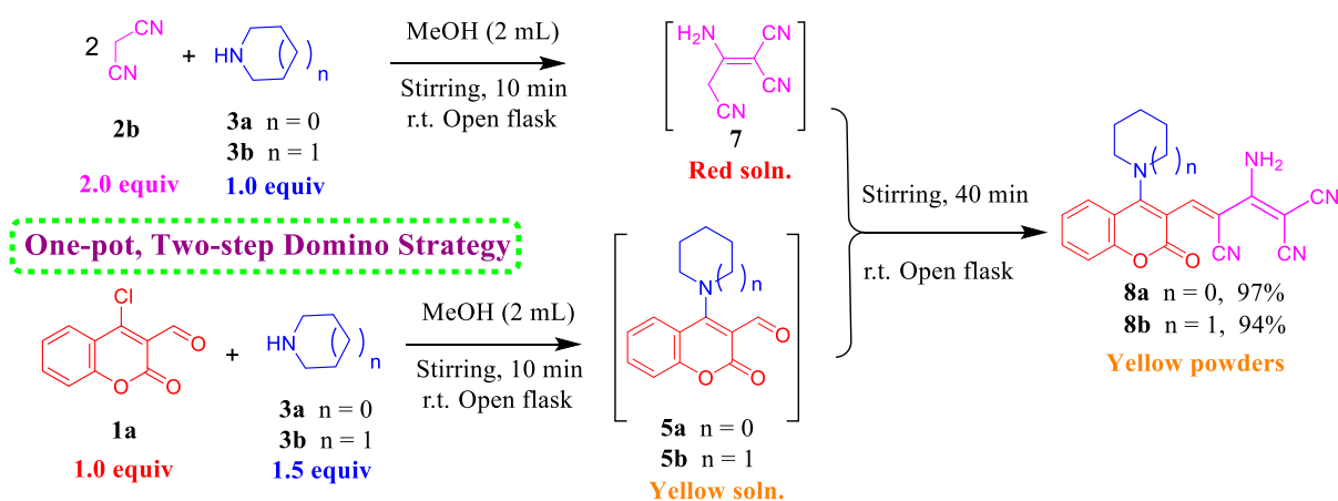
Scheme 5. Previous work by Angelova group and synthesis of 8a,b .
