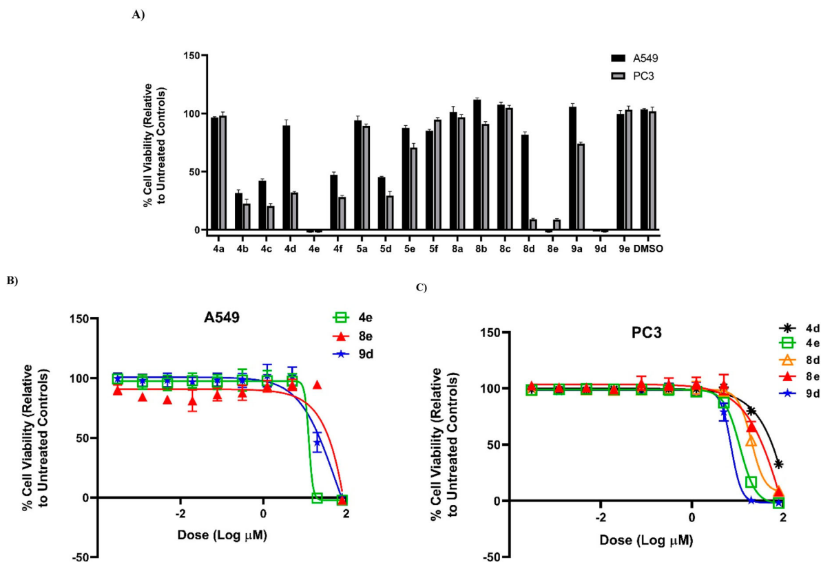
Figure 3. (A) % Viability of A549 (non-small lung) and PC3 (prostate) human cancer cell lines (after 72 h) at 80 \mu\text{M} concentration of compounds 4a–f , 5a , 5d–f , 8a–e , 9a , and 9d–e . (B) Dose–response of compounds 4e , 8e , and 9d against A549 (non-small cell lung) human cancer cell line (72 h). (C) Dose–response of compounds 4d , 4e , 8d , 8e , and 9d against PC3 (prostate) human cancer cell line (72 h).
