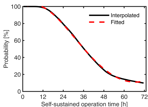
Figure 17. The cumulative distribution for the self-sustained operation duration of the house with an EV at home rated for 20 kWh. threeBuilding resilience was analyzed over a duration of 72 h.
