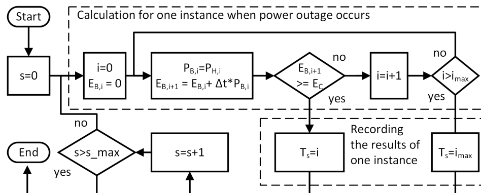
Figure 3. NEW FIGURE–Systematic procedure for the evaluation of building resilience. Simulation is performed for each time step, corresponding to instances for which power outage occurs. The self-sustainment duration is calculated for each instance.
