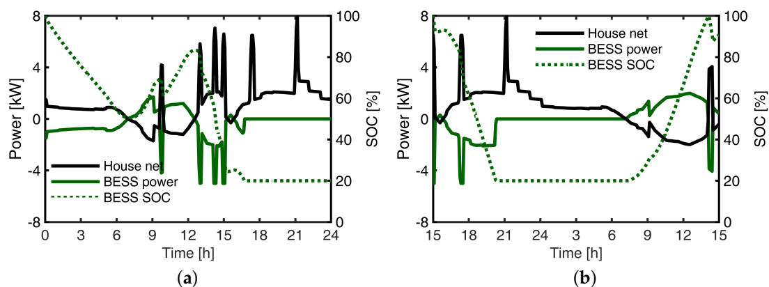
Figure 4. An example of the daily self-sustain case for the reference house when the power outage occurs at (a) midnight and (b) 3 p.m. The BESS covers the residential load in the morning and was charged by surplus solar PV generation throughout the day. As PV power rapidly declined and no longer met the residential load, the BESS discharged until falling to the minimum SOC of 20%. The reference house tends to self-sustain longer when the power outage occurs in the early morning because the BESS could be charged by PV generation during the daytime hours.
