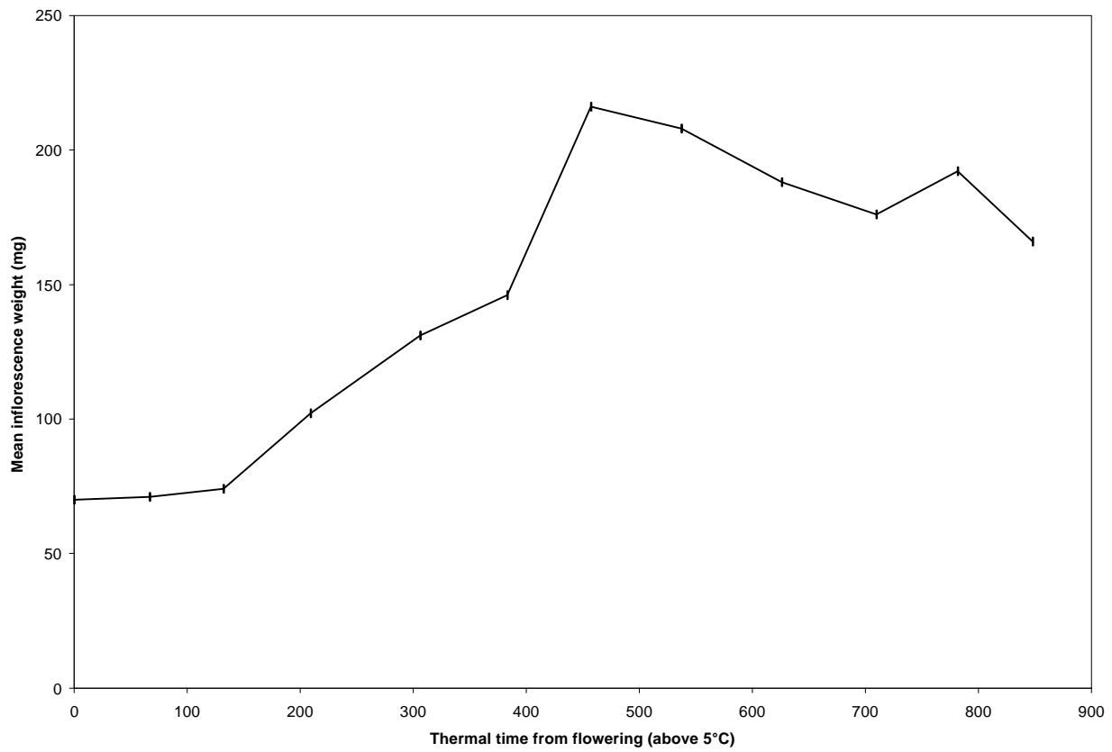
Figure 2 - Inflorescence dry matter change from flowering to seed maturity for Europe.
