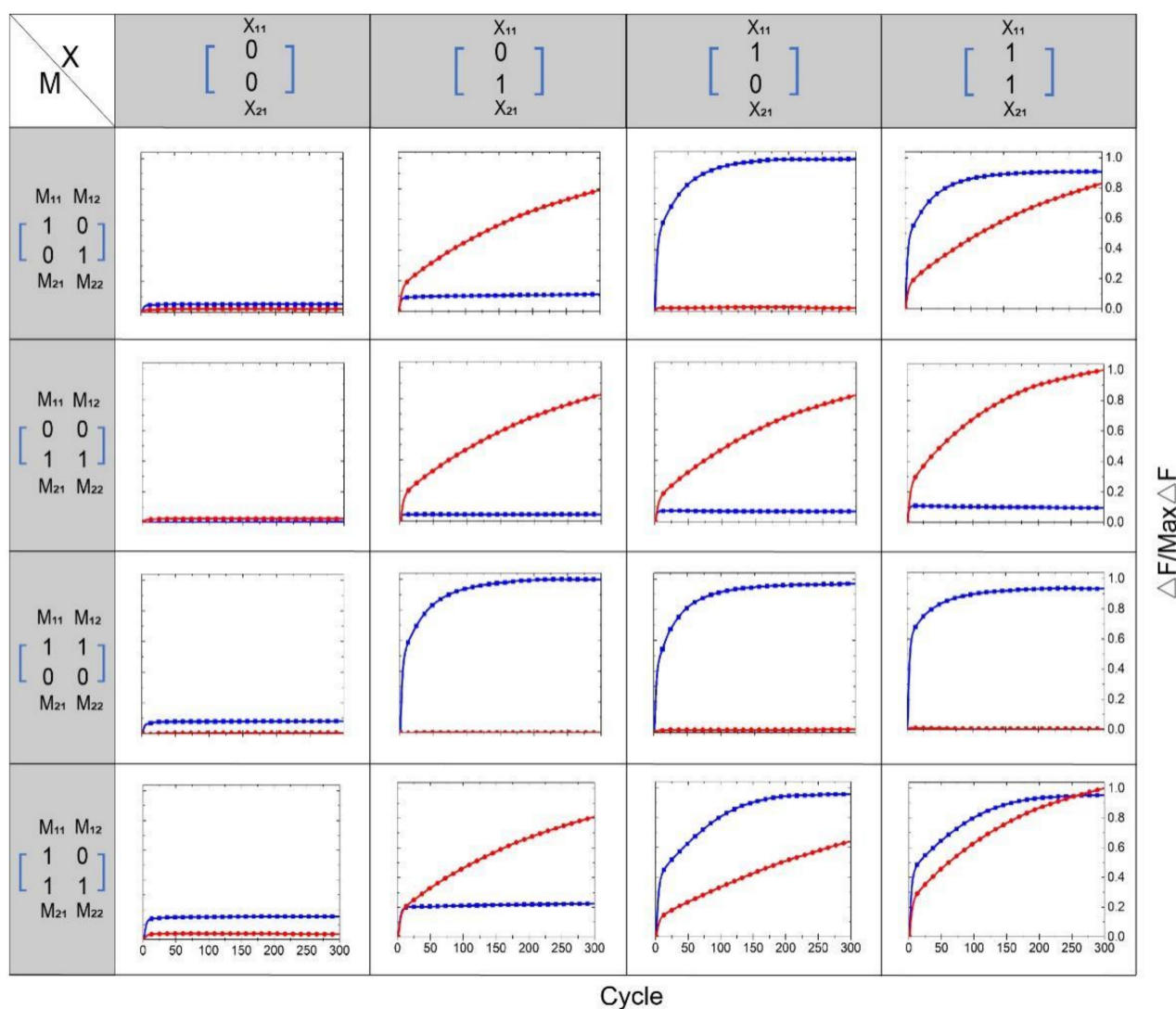
Figure 5. Results of 16 independent experiments. Before adding the element strands of the two matrices, the two DNAses and the two substrate strands of the reporting module are mixed. The sampling interval is 4 min, 300 cycles.
