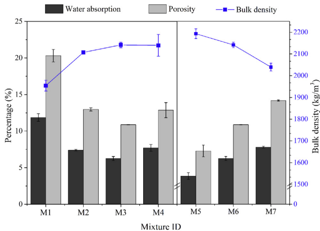
Fig. 7 – Bulk density, water absorption and porosity of OPG M system.
