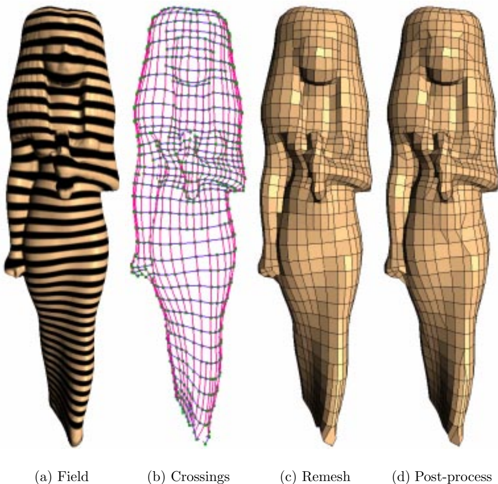
Fig. 7. The 3 stages of mesh generation. First, we build the set of crossings along each flow line. Next we extract a non-conforming mesh from this net of flow crossings. A final post-process produces a conforming mesh composed solely of triangles and quadrilaterals.
