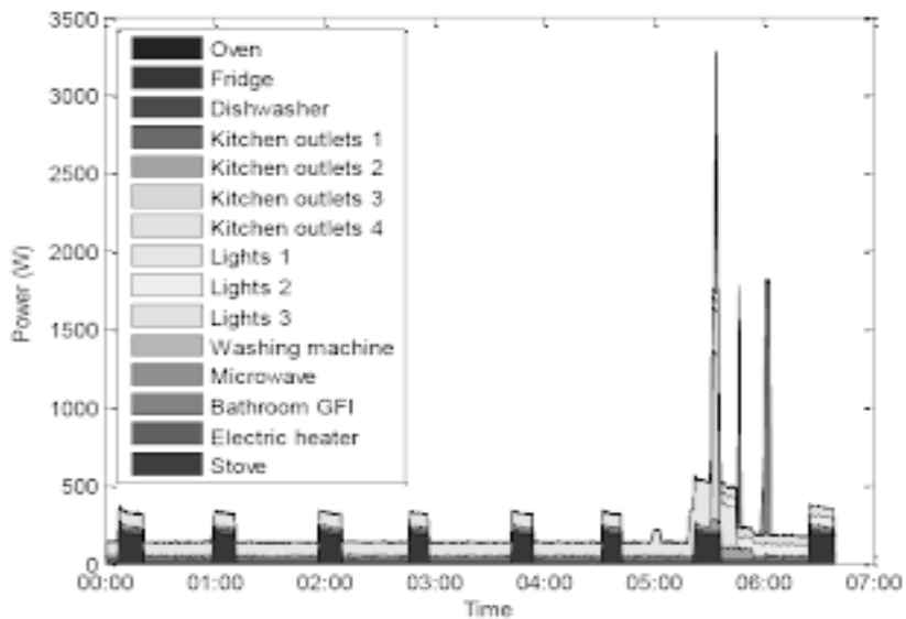
Figure 2: A Household's Power Demand Disaggregated into Appliances 100
