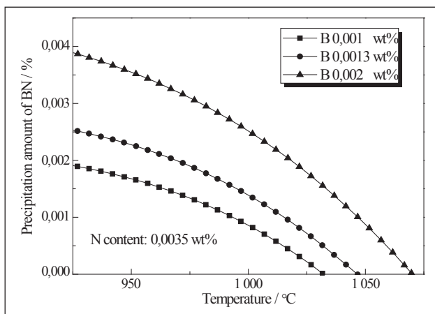
Figure 2 Precipitation amount of BN vs temperature with different boron content
