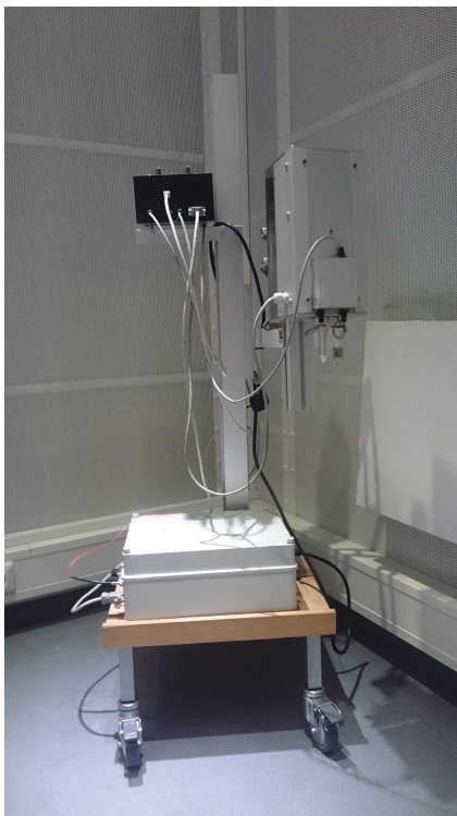
Fig. 1: Vibratory stimulator
