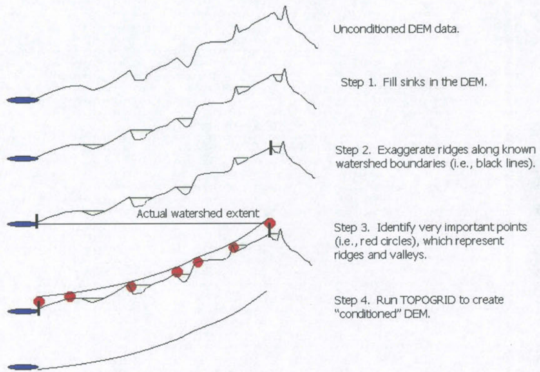
Figure 6. Digital Elevation Model (DEM) conditioning.
