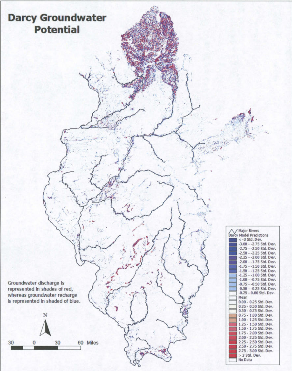
Figure 5. Groundwater potential for Illinois' processing units.
