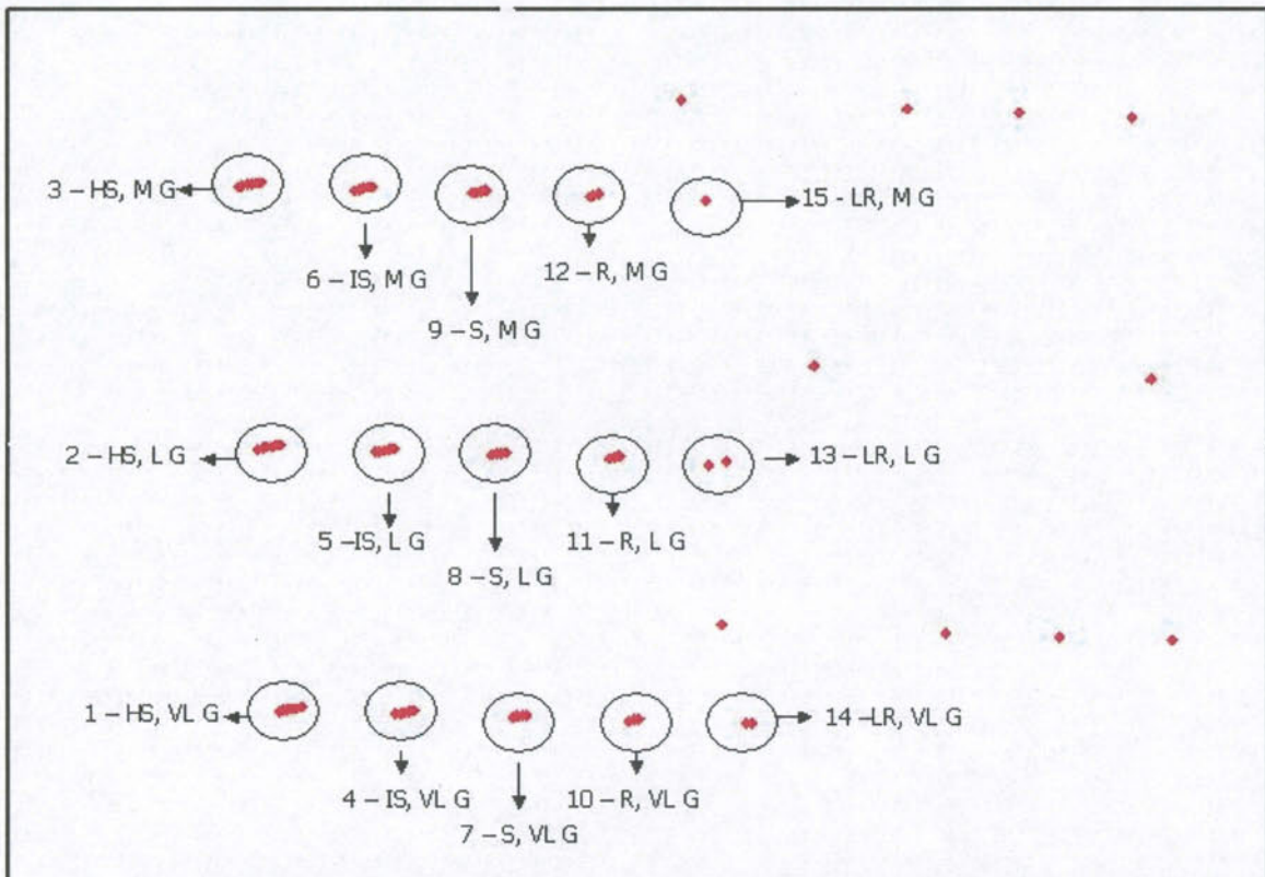
Figure 12. Results from principal components analysis used to identify groupings of stream types. The numbers associated with each grouping refer to the "combo type" in Table 1. Diamonds not included in a grouping had d-link values = 99 and were added to 1 of the other 15 groupings after d-link values were corrected. Text descriptions of each grouping refer to the legends on Figures 13-17. Text codes are as follows: HS=headwater stream, IS=intermediate stream, S=stream, R=river, LR=large river, VLG=very low gradient, LG=low gradient, and MG=moderate gradient.
