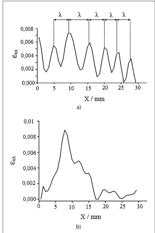
Figure 4 The local elongation \varepsilon_{xx} along the axis of extension during (a) - parabolic strain hardening; (b) - prefracture stage
