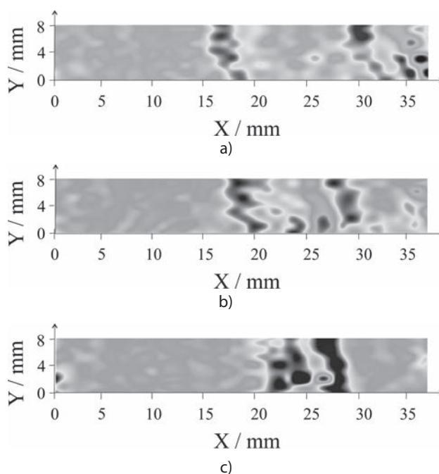
Figure 2 Visualization of Lüders band propagation through the bimetal length at the total deformation of (a) 0,006, (b) 0,008, (c) 0,012
