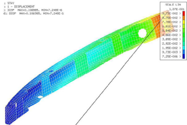
Fig. 2 Predicted displacement of bumper impact beam in case of 5 stays (max.displ.: 1.07\text{ E-01 mm} )
