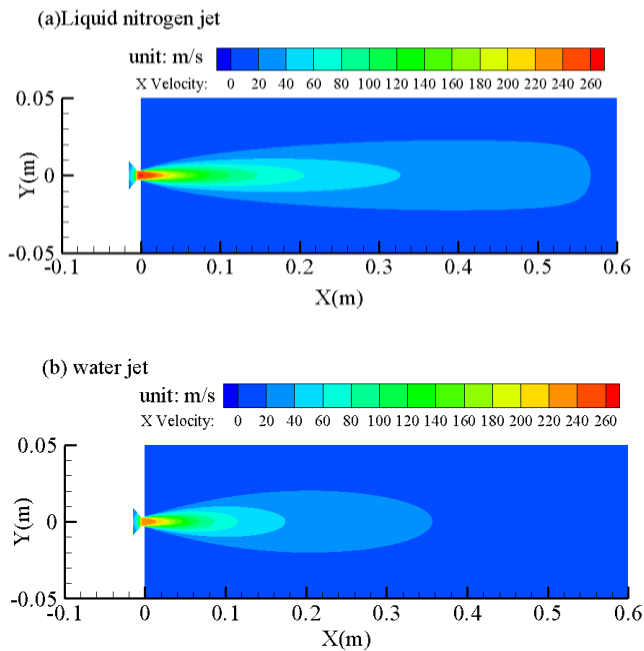
Figure 4. Velocity contours of the liquid nitrogen and water jets in the nearby nozzle.
